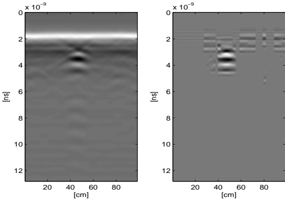
Fig. 4. B-Scan for DeTeC data before and after applied the Gaussianity test algorithm, respectively.
