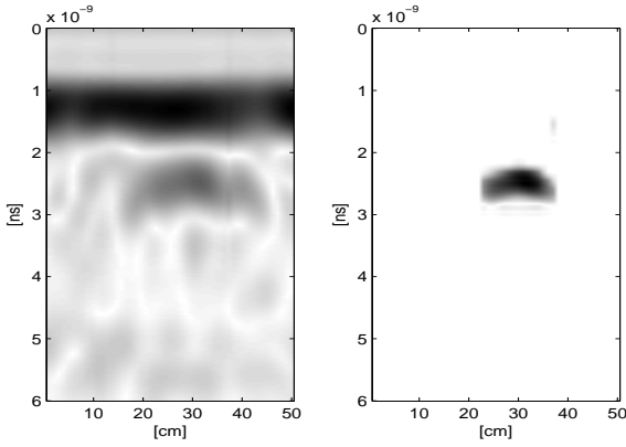
Fig. 3. B-Scan for IESK data before and after applied the Gaussianity test algorithm, respectively.
