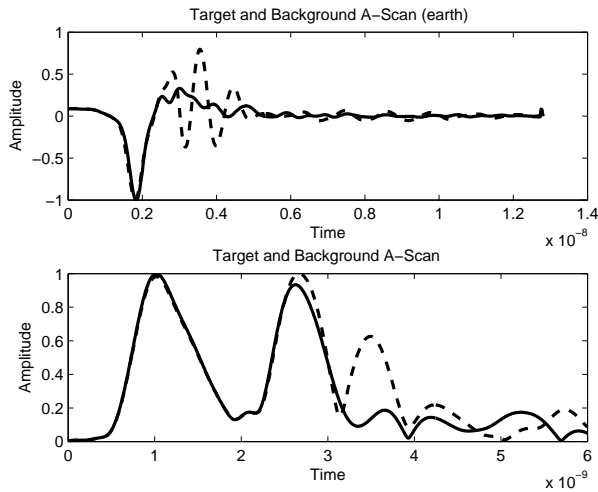
Fig. 1. A scans in the presence (dashed) and absence (solid) of a mine, DeTeC and IESK data, respectively.
