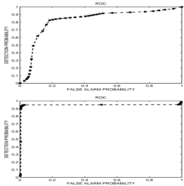
Fig. 5. ROC curve before and after applied Gaussian test, respectively.
