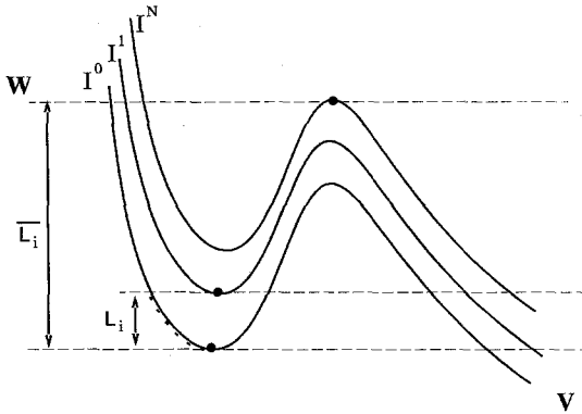
Fig. 6. Defining the domain of the Poincaré map in higher dimensional networks. Relaxation oscillators that receive multiple inputs have trajectories that are defined by several cubic nullclines, each determined by the number and size of synaptic inputs received. The change of a single input may still cause an early jump. The knees of the uppermost cubic ( I^N ) and lower two cubics ( I^0 and I^1 ) define the intervals L_i and \bar{L}_i as in Fig. 4. The set of n -dimensional points for which each oscillator lies in its L_i and at least one oscillator lies at its lower knee, defines the domain of the map \mathcal{P}_L .
