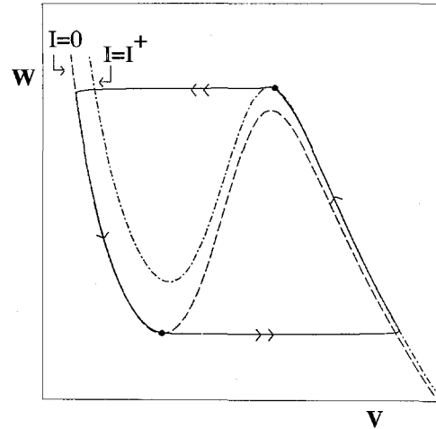
Fig. 3. The limit cycle with input (LCI) for an oscillator is defined by pieces of the left branch of the I = 0 cubic and the right branch of the I = I^+ cubic. The LCI represents the trajectory followed by an oscillator when its onsets and offsets are synchronous with those of the oscillators that provide its input.
