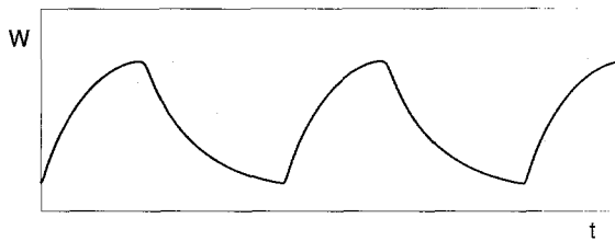
Fig. 5. Slow variable time course for the Morris–Lecar oscillator. The time required to traverse a w interval increases as threshold (a “knee”) is approached. This “scalloped” shape of the time course ( w' \cdot w'' < 0 ) satisfies Hypothesis C.
