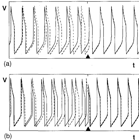
Fig. 9. Synchronization of chains of relaxation oscillators occurs rapidly despite the lower input to the end oscillators of the chain. (a) A “chain” of three Morris–Lecar oscillators ( \epsilon = 0.01 , \alpha = 0.1 ), in which the middle oscillator receives coupling input from its two neighbors and the end oscillators receive only one coupling input. This input difference produces different LCI and different periods for the middle and end oscillators. This difference is demonstrated by starting the oscillators with identical initial conditions and switching the coupling to LCI mode (inputs from self, rather than neighbors). The two end oscillators have the same LCI and thus remain synchronized (traces overlaid), while the middle oscillator drifts. At the mark, LCI coupling is replaced by chain coupling. The relaxation oscillators compensate for differences in input to the end oscillators and the chain synchronizes within a single jump. (b) same as (a) but chain contains 40 oscillators ( \epsilon = 0.001 ). Time course of end oscillators (1,40) and three middle oscillators (2,3,20) are shown. In LCI mode the ends and middle drift apart, but rapidly synchronize when chain coupling is activated.
