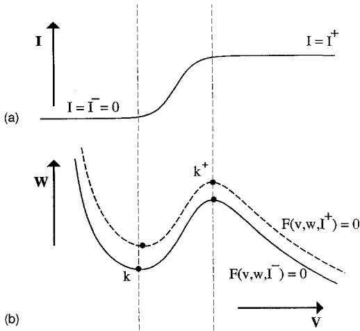
Fig. 2. Heaviside coupling. (a) shows a sigmoidal coupling function, I(V) , for which the non-constant ranges of the function lie in the middle branch of the cubic nullcline (shown in (b)). Since the phase-plane trajectory hugs the outer branches and rapidly jumps between these branches, the coupling function assumes one of two constant values, I^- or I^+ , determined by the branch on which the input oscillator lies. I^- and I^+ define different cubic nullclines with the I^+ nullcline shifted upward, possibly with a change of shape as shown in (b). The trajectory of a coupled pair of identical oscillators can be described by these two cubics and the rapid transitions between them. The local extrema or “knees” are important transition points.
