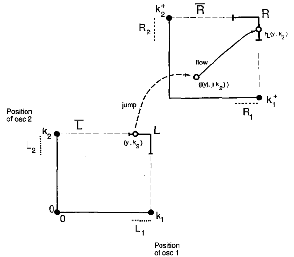
Fig. 7. One half of the Poincaré map for a pair of coupled oscillators. L and R (solid line corners) represent the sets of points for which both oscillators make simultaneous jumps in the next instant. \bar{L} and \bar{R} (dashed line corners) define the supersets of L and R for which at least one oscillator is at the jump threshold. After a synchronous jump from L (or R ), oscillators then flow until they lie in \bar{R} (or \bar{L} ). A synchronous jump and the subsequent flow therefore describe a map from L to \bar{R} (or from R to \bar{L} ). The intervals R_i and L_i are as in Fig. 2.
