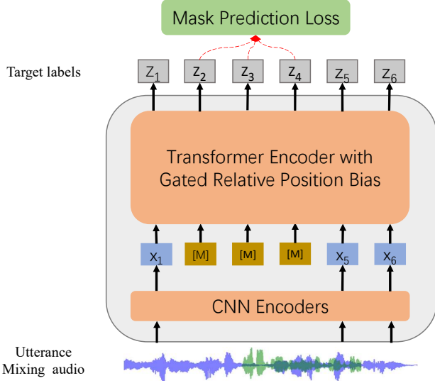
Fig. 1. Model Architecture.
