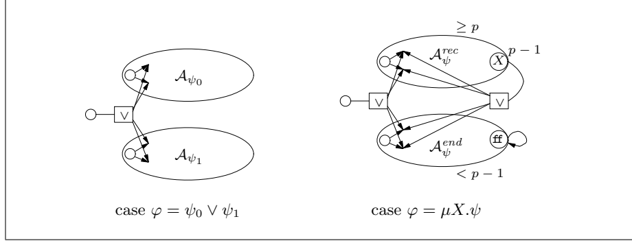
Fig. 1. Illustrations of the translation from \mu\text{TL} to WAPA.
