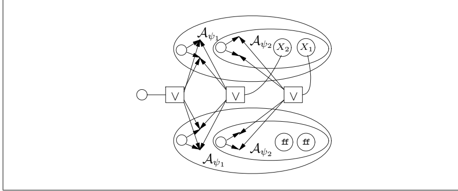
Fig. 2. Simultaneously translating fixpoint formulas into WAPAs.
