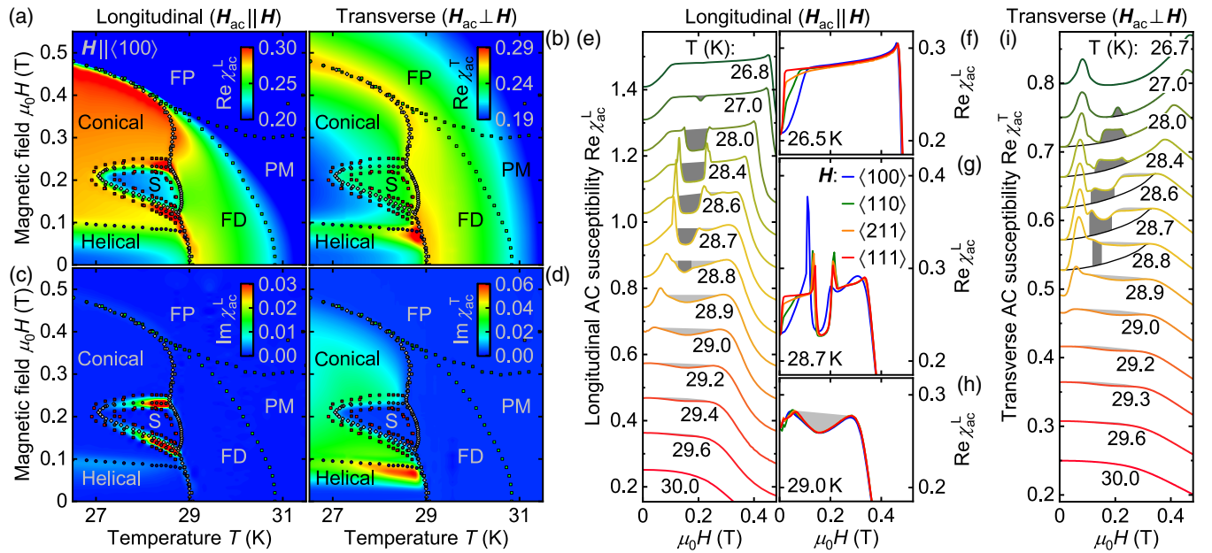
FIG. 1. Longitudinal and transverse ac susceptibility. (a)–(d) Color maps of the real and imaginary parts of the longitudinal and transverse susceptibilities, \chi_{ac}^L and \chi_{ac}^T , for a field along \langle 100 \rangle after zero-field cooling. Data points are inferred from temperature (light colors) and field sweeps (dark colors) of the differential susceptibility dM/dH (circles), \chi_{ac}^L (squares), and specific heat measurements (diamonds); see text for details. The following six regimes may be distinguished: helical ( H ), conical ( C ), skyrmion lattice ( S ), fluctuation disordered ( FD ), paramagnetic ( PM ), and field-polarized ( FP ). (e) \text{Re } \chi_{ac}^L as a function of field for different temperatures. Dark and light shadings indicate contributions that arise from the skyrmion lattice state and skyrmionic fluctuations, respectively. Data have been offset for clarity. (f)–(h) \text{Re } \chi_{ac}^L for different field directions and temperatures well below, around, and just above T_c . Isotropic behavior is observed in the regime without static order. (i) \text{Re } \chi_{ac}^T as a function of field for different temperatures.
