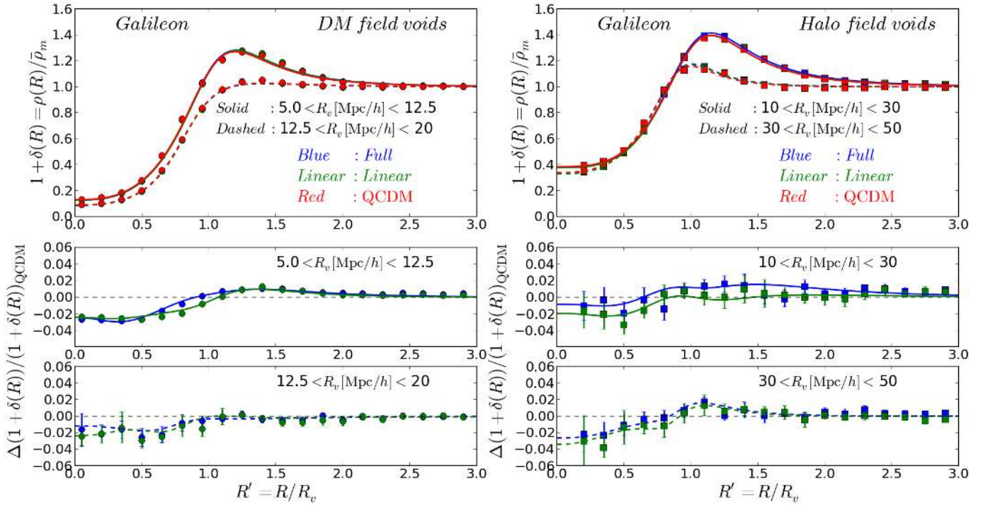
FIG. 3. Void density profiles, \rho_m/\bar{\rho}_m = 1 + \delta , for the DM density field (circles, left panels) and halo density field (squares, right panels) voids found in the simulations of the three Galileon model variants (distinguished by the different colors, as labelled), plotted as function of the scaled radius R' = R/R_v . The solid (dashed) lines show the best-fitting density profiles, using the formula of Eq. (26), for the bin of smaller (larger) void sizes, as labelled. The bottom panels show the relative difference to QCDM. The errorbars depict the variance across the five realizations of each variant.
