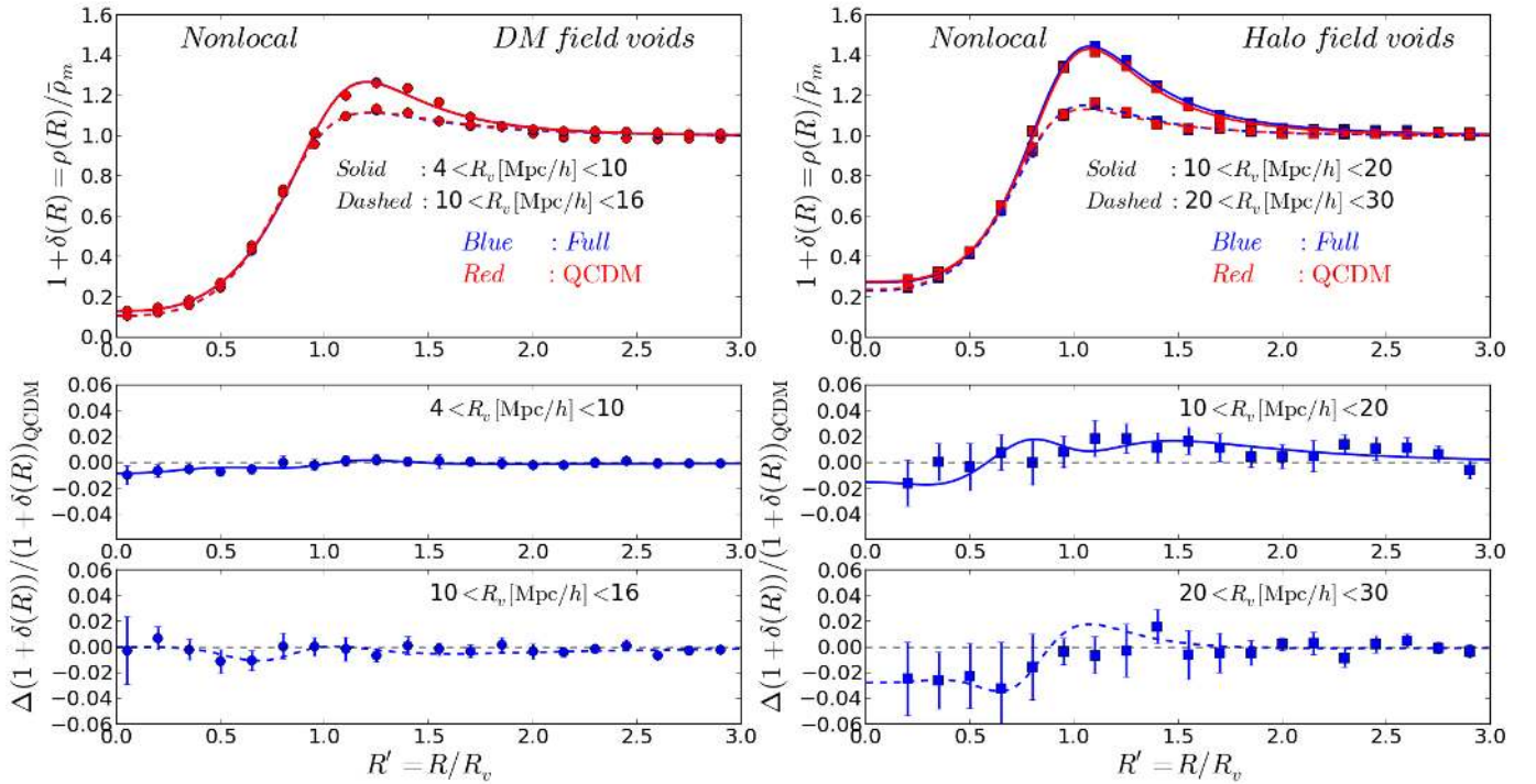
FIG. 4. Same as Fig. 3 but for the Nonlocal gravity model.
