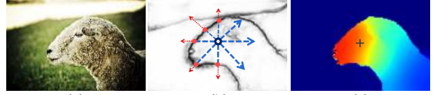
Figure 4. Deriving pairwise semantic affinities from a class boundary map. (left) Input Image. (center) A class boundary map. (right) Label propagation from the center after random walks.
