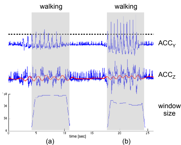
Fig. 7. Adaptive filter for artefact compensation while walking slowly (a) and fast (b). Vertical acceleration signal ( ACC_Y ) and threshold (dashed line) for detecting walking activity. Horizontal acceleration signal ( ACC_Z ) and first derivative for calculating the step length. The window size used by the median filter and tuned to the walking pace is shown at the bottom.
