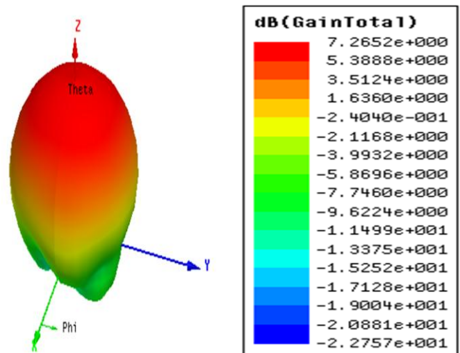
Figure 3 3-D Radiation pattern of antenna
