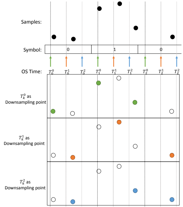
Figure 11: Downsampling example on real samples. Each T_0^j determines a sampling sequence, PIXEL chooses T_0^1 since it has the best decoding SNR.
