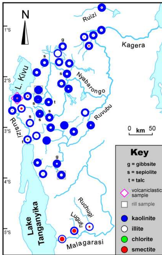
Figure 4. Geographic distribution of clay minerals (circle diameters are proportional to relative mineral abundances). Kaolinite, the typical product of equatorial weathering, is dominant through most of the study area. Smectite characterizes volcaniclastic as well as plutonic and metamorphic mud, from the South Kivu region and Rusizi basin to the lower Kagera, Ruizi, and Malagarasi Rivers draining savannah lowlands of Rwanda, Uganda, and Tanzania. Illite may be locally dominant in muds derived from Mesoproterozoic meta-sediments in Burundi and Rwanda, where gibbsite was occasionally detected. Minor chlorite frequently occurs in muds of Burundi rivers draining toward Lake Tanganyika.
