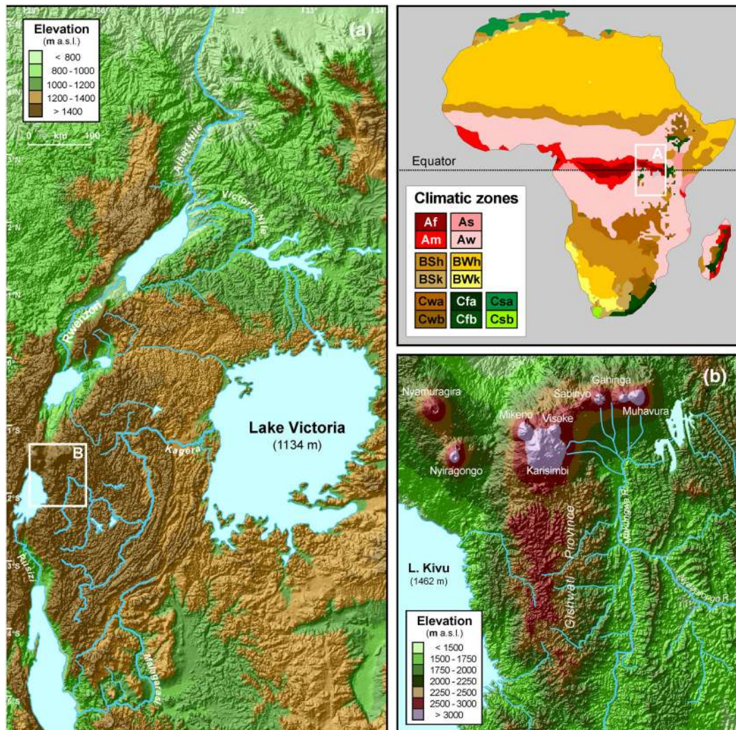
Figure 1. Climate and relief in equatorial Africa. (a) Topography and drainage patterns in the study area. (b) Virunga volcanic field and Gishwati Province (northern part of the Tanganyika-Kivu rift shoulder). Shown in the upper right panel is the distribution of climatic zones (Köppen-Geiger classification after Kottek et al. [2006]). Main climates: A = equatorial; B = arid; C = warm temperate. Precipitation: W = desert; S = steppe; f = fully humid; s = summer dry; w = winter dry; m = monsoonal. Temperature: h = hot arid; k = cold arid; a = hot summer; b = warm summer.
