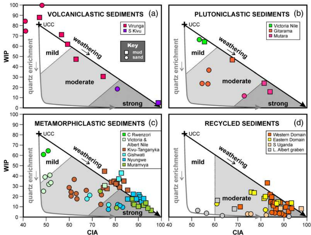
Figure 9. Discriminating first-cycle and polycyclic sediments with chemical indices. Because quartz dilution affects strongly WIP but not CIA, the CIA/WIP plot readily reveals quartz enrichment in sediments. The relationship between CIA and WIP is linear for first-cycle muds as well as for quartz-poor volcaniclastic sands (a), whereas with increasing weathering intensity, quartz enrichment causes a marked decrease of WIP in plutoniclastic and metamorphiclastic sands (b, c). Sediments recycled from quartzose sediments and meta-sediments display low WIP even where weathering is limited, as revealed by low CIA (d). Sands, largely resulting from physical erosion, invariably display lower CIA than muds, the ultimate product of chemical weathering.
