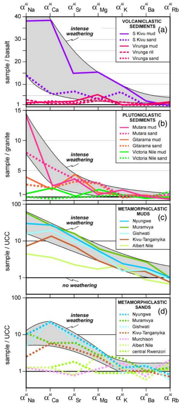
Figure 7. Systematic differential depletion in alkali and alkaline-earth metals. In humid Nyungwe, Muramvya, and Gishwati rift highlands, as well as in the South Kivu and Mutara Provinces, \alpha^{Al} values for Na and Ca typically range from 5 to 20 in sands and from 10 to 50 in muds, whereas for Ba and Rb, they are invariably <5 . In the Virunga Province and Victoria Nile at Itanda Falls, both sands and muds are virtually unweathered ( \alpha^{Al} \sim 1 for all elements). Gray areas are empirical envelopes for intense equatorial weathering.
