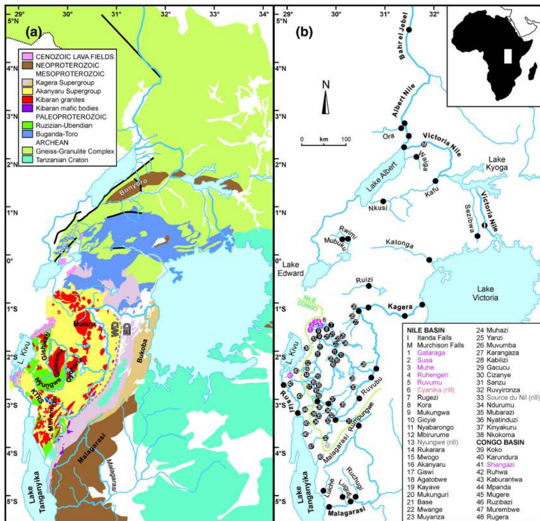
Figure 2. The western branch of the East African Rift with identified sedimentary provinces. (a) Geological sketch map (compiled after Schlüter [2008], Fernandez-Alonso [2007], and other sources cited in text). KTRS = Kivu-Tanganyika rift shoulder. WD, ED = Western and Eastern Domains [Tack et al., 2010]. (b) Studied rivers and sampling sites.
