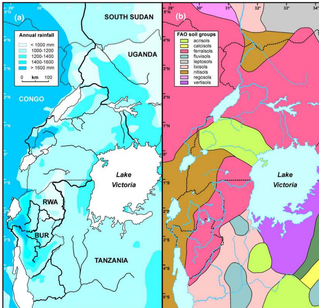
Figure 3. Climate and soil types in equatorial central Africa. (a) Rainfall map. (b) Soil map (distribution of soil groups as classified by the Food and Agriculture Organization, www.britannica.com/bps/media-view/19257/0/0/0 ). RWA = Rwanda; BUR = Burundi.
