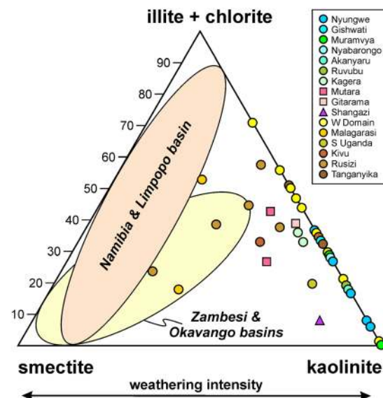
Figure 6. Weathering intensity as revealed by clay-mineral assemblages. Kaolinite is the predominant clay mineral throughout equatorial central Africa, in sharp contrast with drier tropical Southern Africa (Namibia and Limpopo basin) [own data]. Only in the Zambesi and Okavango river systems, sourced in humid sub-equatorial Angola and Zambia, the kaolinite/smectite ratio may approach that of muds produced in drier areas of NW Tanzania and W Burundi (Malagarasi and Rusizi basins).
