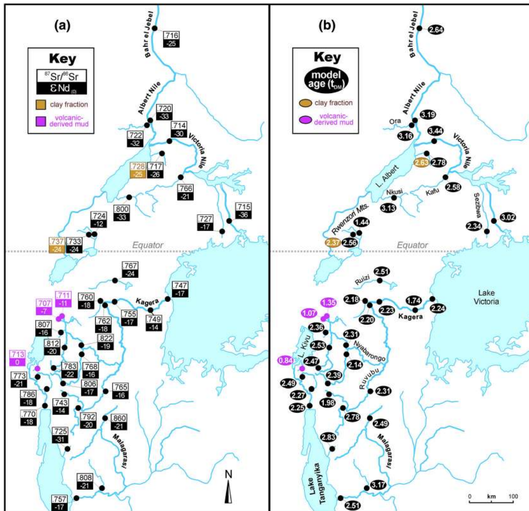
Figure 5. Isotopic signature of muds. (a) ^{87}\text{Sr}/^{86}\text{Sr} ratios and \epsilon\text{Nd}_{(0)} . Victoria and Albert Nile muds display lower ^{87}\text{Sr}/^{86}\text{Sr} and more negative \epsilon\text{Nd}_{(0)} than mud in the Kagera basin, reflecting lack of sediment connection across Lake Victoria. (b) Model mantle derivation ages ( t_{\text{DM}} ). Paleoproterozoic model ages characterize sediments all along the rift shoulders from Burundi to the Rwenzori mountains. Instead, Archean model ages characterize muds of NW Tanzania and Uganda directly or indirectly derived from the Tanzania and Congo Cratons. Much younger Proterozoic ages characterize muds produced in Neogene volcanic fields.
