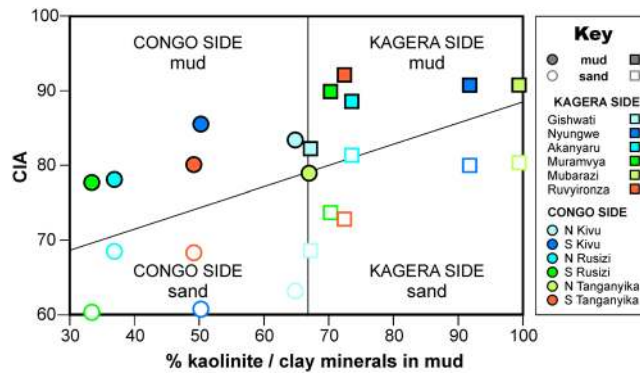
Figure 8. Contrasting weathering conditions on opposite rift-shoulder flanks. Clay mineralogy and chemical indices consistently reveal more intense weathering in hot-humid forested highlands on the eastern Kagera-Nile side of the divide, where slopes are milder, and time for weathering longer, than along the steep inner flank and drier axis of the rift (Congo side). Note that CIA values are invariably higher for mud samples than for corresponding sand samples.
