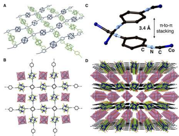
Figure 2. (A) SCXRD showing the woven structure formed from building blocks 1 and 2. The triethyl phosphine groups and hydrogen atoms have been removed to clarify the view. (B) The templation utilizes the 4-fold axis of \text{Mo}_6\text{O}_{19}^{2-} . (C) \pi -to- \pi interactions holding the strands in registry. (D) Side view of the crystal packing showing the cationic and anionic layers ( a -axis). Note that the ethyl groups from the phosphine subunits, which envelop the surface of the templating Lindqvist nanooxides with directional C–H \cdots O hydrogen bonds, have been omitted in B and D to clarify the view.
