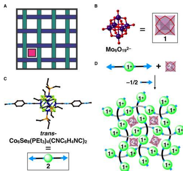
Figure 1. (A) Two-dimensional box weave. The magenta square represents a template for the box weave. (B) Lindqvist dianion \text{Mo}_6\text{O}_{19}^{2-} 1 and its polyhedral representation. (C) \text{Trans-Co}_6\text{Se}_8(\text{PEt}_3)_4(\text{CNC}_6\text{H}_4\text{NC})_2 ( 2 ) and cartoon. (D) Two-step assembly between the \text{Mo}_6\text{O}_{19}^{2-} template and [\text{Co}_6\text{Se}_8(\text{PEt}_3)_4(\text{CNC}_6\text{H}_4\text{NC})_2]^{1+} to form a box weave.
