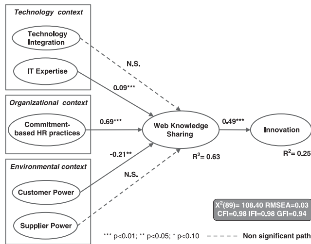
Figure 2 Empirical results.
