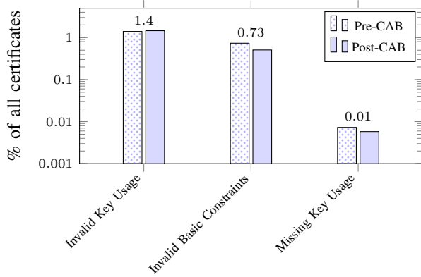
Fig. 7. Extension Violations in Intermediate Certificates
