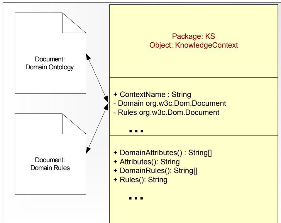
Figure 4. Modular Knowledge Context
