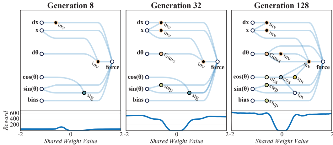
Figure 4: Development of Weight Agnostic Neural Network Topologies Over Time Generation 8: An early network which performs poorly with nearly all weights. Generation 32: Relationships between the position of the cart and velocity of the pole are established. The tension between these relationships produces both centering and swing-up behavior. Generation 128: Complexity is added to refine the balancing behavior of the elevated pole.
