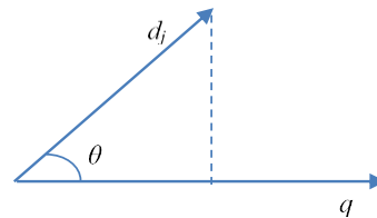
Figure 2. Vector representation
