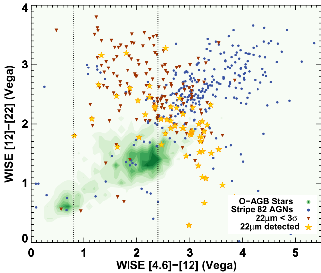
Figure 8. [4.6]–[12] vs. [12]–[22] WISE colors for oxygen-rich AGB stars (green color scale; Suh & Kwon 2011), Stripe 82 “strong” AGNs (blue points; E. Glikman et al. 2017, in preparation), 22 \mu\text{m} non-detected (dark triangles), and 22 \mu\text{m} -detected post-starbursts (yellow stars) from the extended source sample of 158. The IRTZ is represented by black dotted lines. As was shown in Figures 1 and 2, post-starbursts fall in the infrared transition zone. Many post-starbursts exhibit [12]–[22] colors consistent with AGNs.
