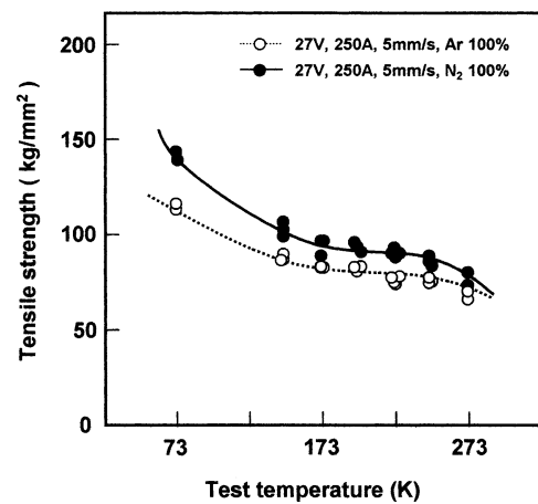
Fig. 16. Effect of temperature on the tensile strength of SUS 316 welds made in \text{N}_2 shielding gas.
