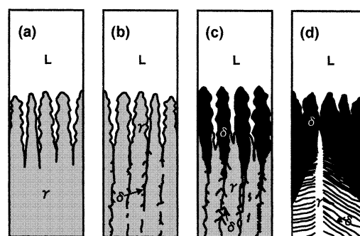
Fig. 8. Schematic illustration of solidification model for austenitic-ferritic weld metals: (a) A mode, (b) AF mode, (c) FA mode, (d) F mode.
