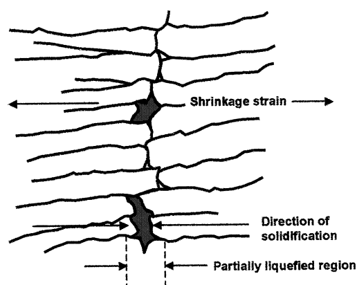
Fig. 11. Schematic illustration of mechanism for solidification cracking.
