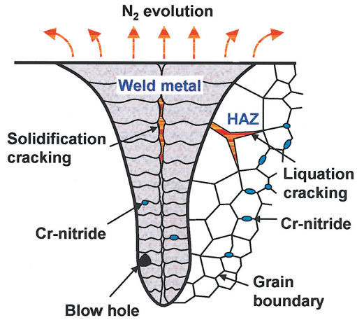
Fig. 1. Schematic illustration of high nitrogen steel weld.
