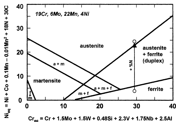
Fig. 9. Modified schaffler diagram for stainless steel weld metal.
