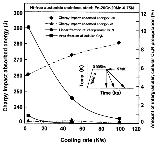
Fig. 18. Effect of cooling rate on Charpy impact absorbed energy and amount of intergranular, cellular \text{Cr}_2\text{N} precipitation.
