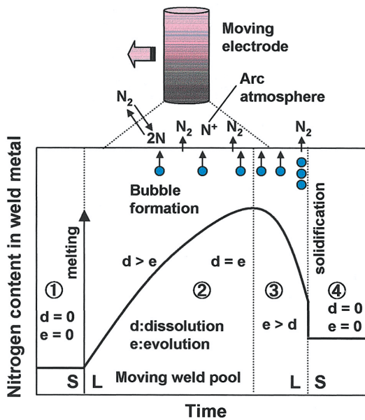
Fig. 2. Schematic illustration of the weld metal nitrogen content under a moving welding arc in an atmosphere containing nitrogen gas ( N_2 ): Stage 1: premelting stage, Stage 2: arc melting with dissolution dominating. Saturation ( i.e. , d=e ) may or may not be reached. Note that d=e is a time independent condition and not necessarily a thermodynamic equilibrium condition, Stage 3: Weld metal cooling (still liquid) with decreasing saturation solubility and evolution dominating (bubble evolution may prevail), Stage 4: Solidification with step change in solubility and consequent rejection of nitrogen with excess causing porosity, accompanying nitrogen in solid solution.
