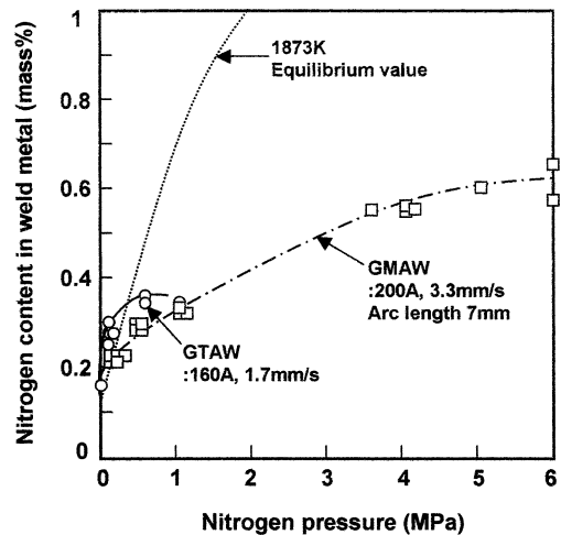
Fig. 4. Nitrogen absorption of SUS316 weld metal under GTA and GMA welding processes.
