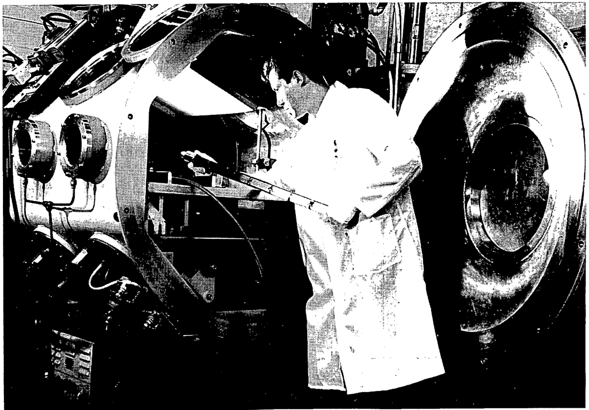
Figure IX-7. - Vacuum purged weld chamber.
