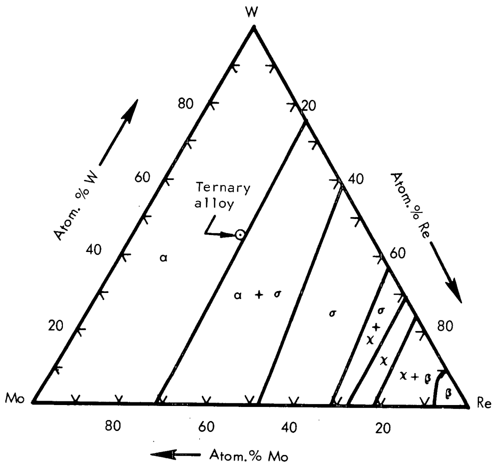
Figure IX-3. - Tungsten-rhenium-molybdenum ternary phase diagram: 1830 o F isotherm (ref. 4).
