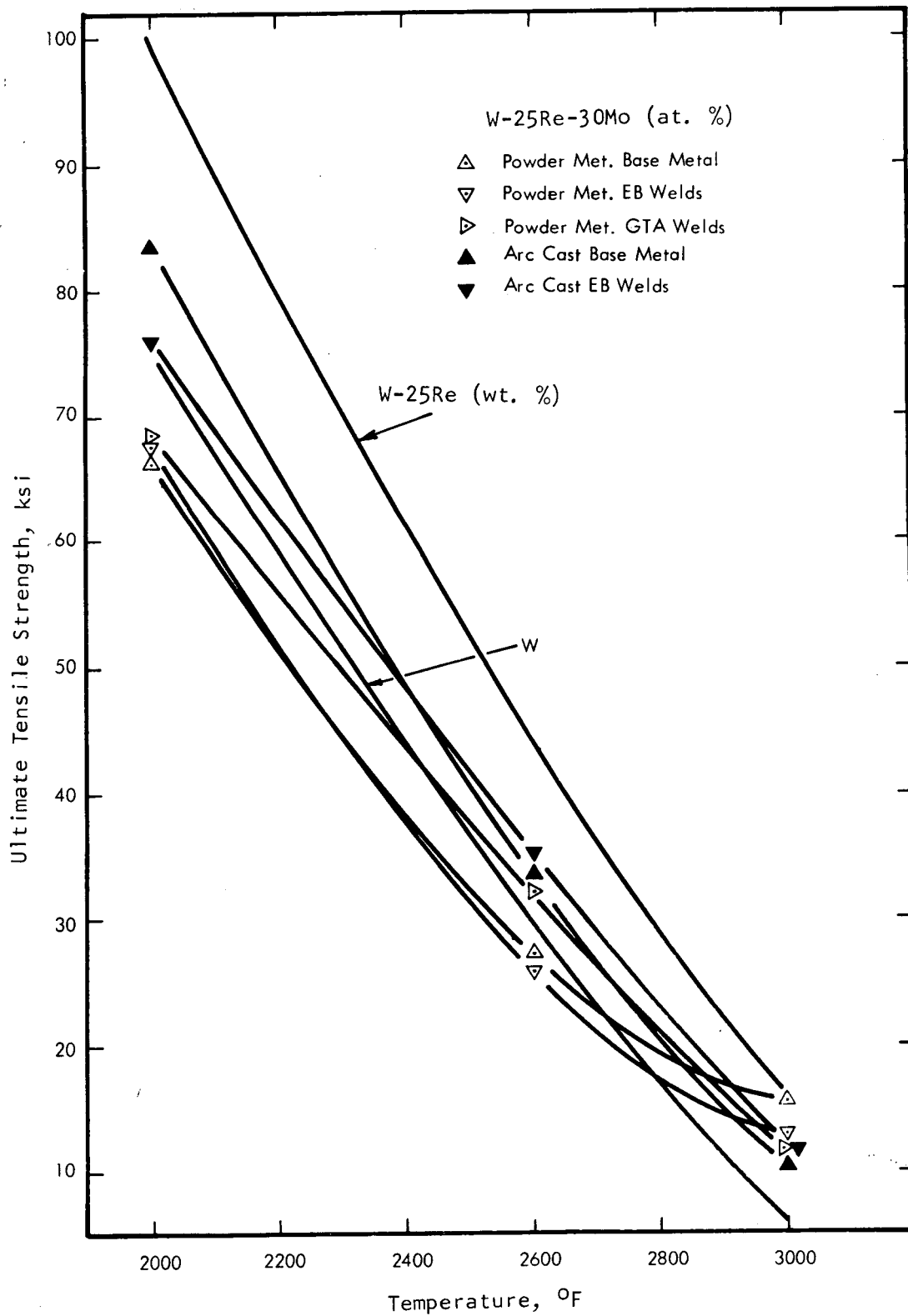
Figure IX-4. - Elevated temperature ultimate tensile strength of tungsten-base alloys.
