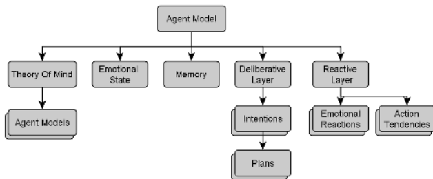
Figure 3: FATiMA extended with ToM
