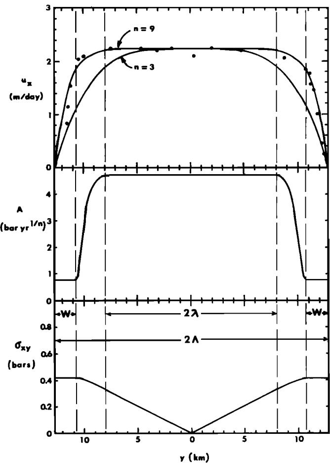
Fig. 23. The Byrd Glacier velocity data related to viscoplastic instability and strain softening alongside an ice stream. Longitudinal surface velocities u_x across section Y-Y' in Figure 2, reported by Swithinbank [1963] and shown as solid circles, are compared with theoretical curves for homogeneous flow, in which the rigidity parameter A is constant and the shear stress \sigma_x , varies linearly across the ice stream. Agreement is poor for n = 3 , the measured viscoplastic parameter of ice, and fair for n = 9 , a nearly plastic viscoplastic parameter. Agreement is best for n = 3 if A and \sigma_{xy} vary as shown, which is expected if viscoplastic instability creates a four-pole ice fabric in zone 2\lambda , a single-pole ice fabric in zones W , and transitional ice fabrics in zones \Lambda - \lambda - W . As is shown in Figure 4, strain softening is much more pronounced in a single-pole fabric than in a four-pole fabric.
