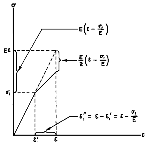
Fig. 7. The perfect elastic-plastic uniaxial flow curve for the bicrystal loaded in Figure 5b after crystal 1 has yielded but before crystal 2 has yielded.
