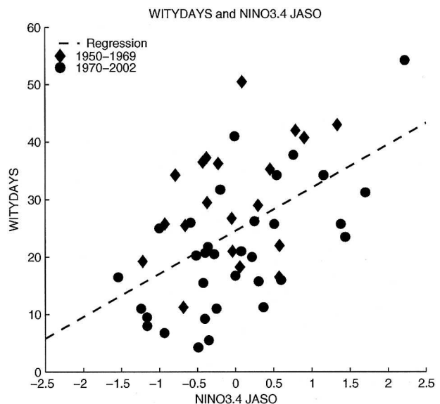
FIG. 10. Same as in Fig. 2, but for weighted number of intense typhoon days per year and Niño-3.4 (°C).
