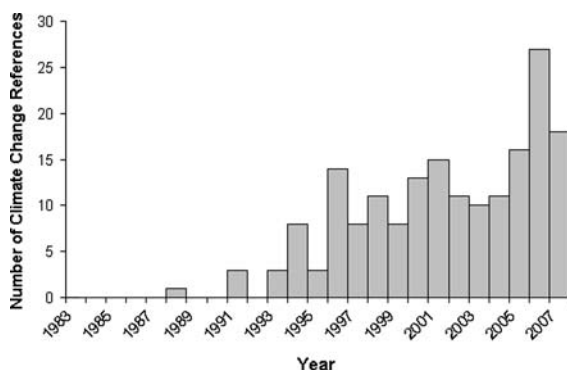
Fig. 2 Climate change references by year
