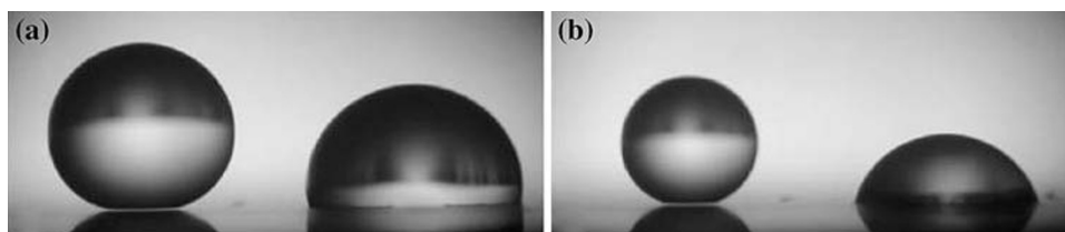
Fig. 6 Illustration of the difference between the Cassie–Baxter and Wenzel states: (a) after deposition of the liquid drops on the surface, (b) after evaporation [24]. Reprinted with permission from [24]. Copyright 2007 Royal Society of Chemistry
