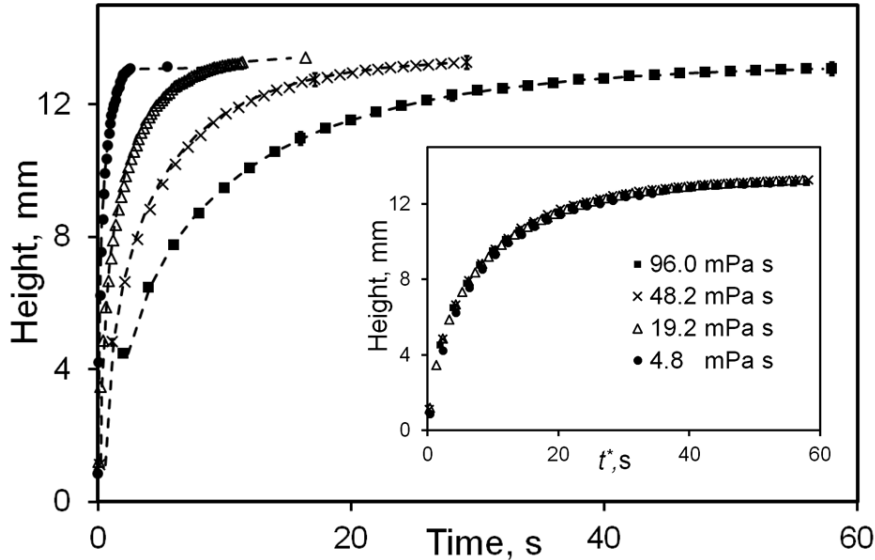
Figure 11. The effect of viscosity on capillary rise for the 600 \mu\text{m} square tube. The dashed lines are the expected rise obtained by taking the fitted value of a for the 96.0 \text{ mPa s} sample and scaling it according to the ratio of viscosities. The inset shows the data scaled for viscosity. The scaled time t^* = 96t/\eta .
