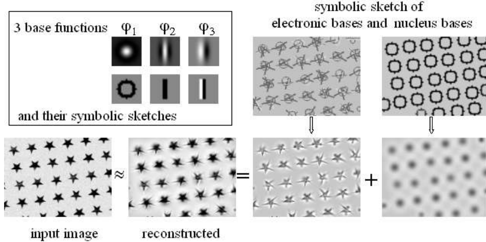
Fig. 8. Reconstructing a star pattern by two layers of bases. An individual star is decomposed into a LoG base in the upper layer for the body of the star plus a few other bases (mostly G_{\cos} , G_{\sin} ) in the lower layer for the angles.
