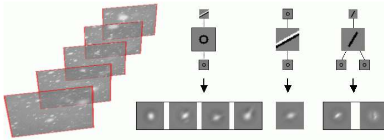
Fig. 12. The texton templates for the snow pattern learned from a movie sequence. The three types of templates for textons and corresponding image appearances.
