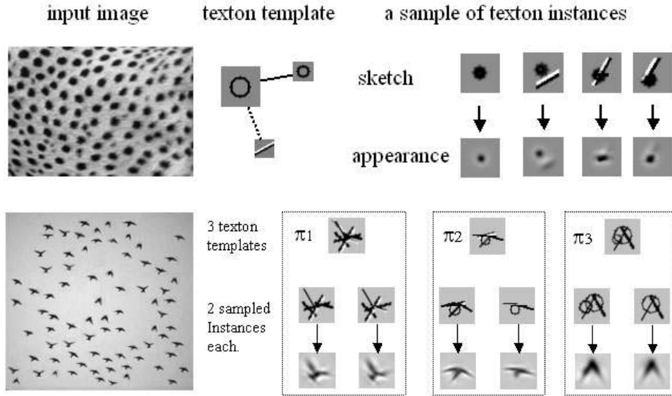
Fig. 10. The texton templates for the cheetah (flying bird) patterns, and a sample of typical texton instances — the sketches (1st row) and image appearances (2nd row)
