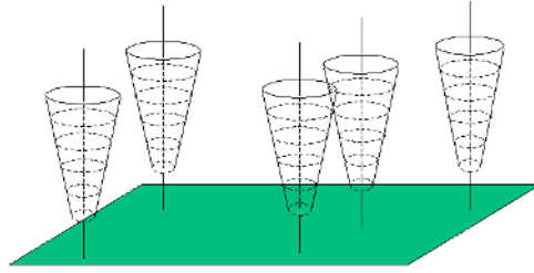
Fig. 2. At each pixel, a pyramid (cone) of filters at various scales and orientations are convolved with the image to extract a feature vector.
