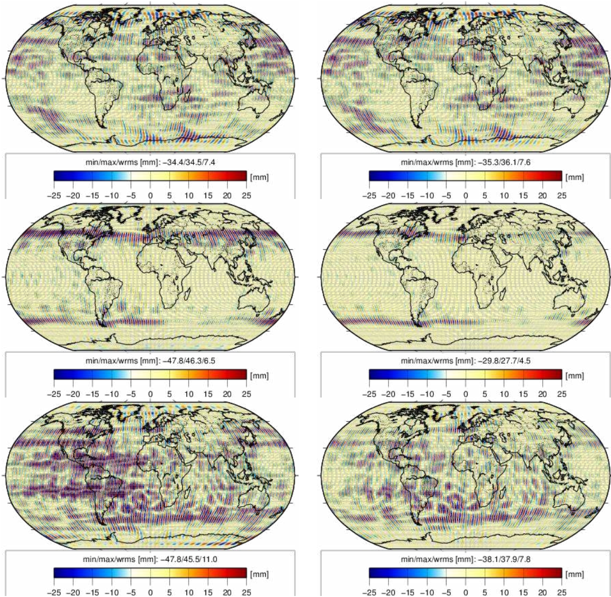
Fig. 11 Spatial difference between simulated (“true”) and recovered gravity fields in terms of unfiltered geoid heights for MWI (left) and LRI (right) derived gravity models for May 2021 in case of ACC errors only (top), ocean tide errors only (middle) and AO errors only (bottom). Statistics show minimum, maximum and wRMS of errors
