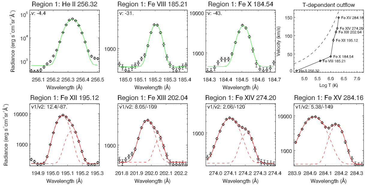
Fig. 10.— Line profiles averaged over region 1 marked in Figure 3. The diamonds, error bars, line styles and colors are the same as in Figure 7. The velocities ( v ) derived from the single (SGF) and double ( v_1 & v_2 for the two components) Gaussian fits are shown in each panel of line profile. Also shown is the temperature dependent outflow velocity and the adiabatic sound speed (dashed curve in the upper right panel).
