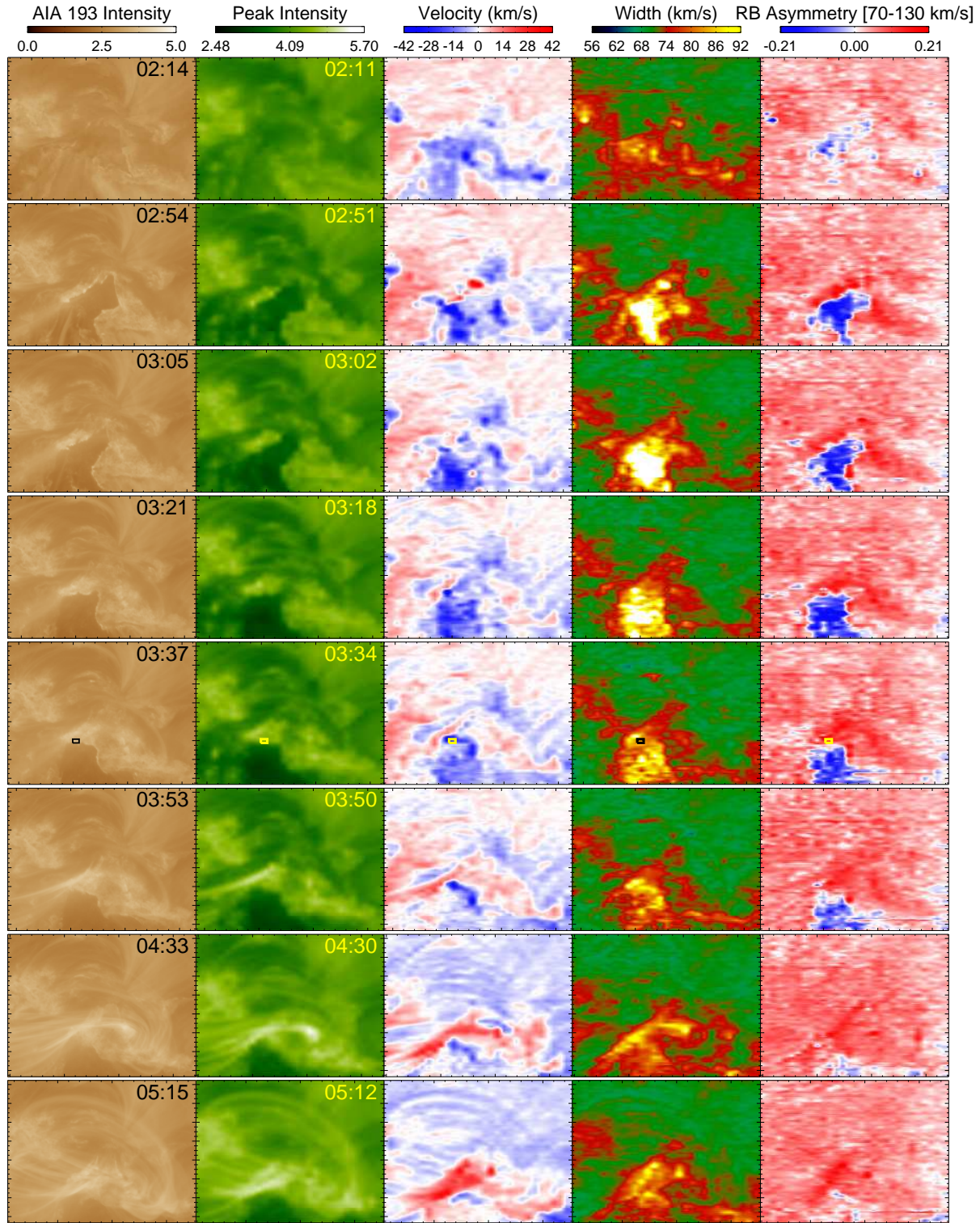
Fig. 4.— Evolution of AIA 193Å intensity and EIS Fe XII 195.12Å line parameters (peak intensity, velocity and width derived from the single Gaussian fit, and the average RB_P asymmetry in the velocity interval of 70-130 km s -1 ) in the 2011 Jun 21 observations. The time of the AIA observation and the beginning time of each EIS scan are indicated in the corresponding intensity images. The rectangular region marks the locations where line profiles are averaged and presented in Figure 11. The size of the FOV is about 175'' × 152''. A movie (m4.mpeg) showing the evolution of AIA 171Å is available online.
