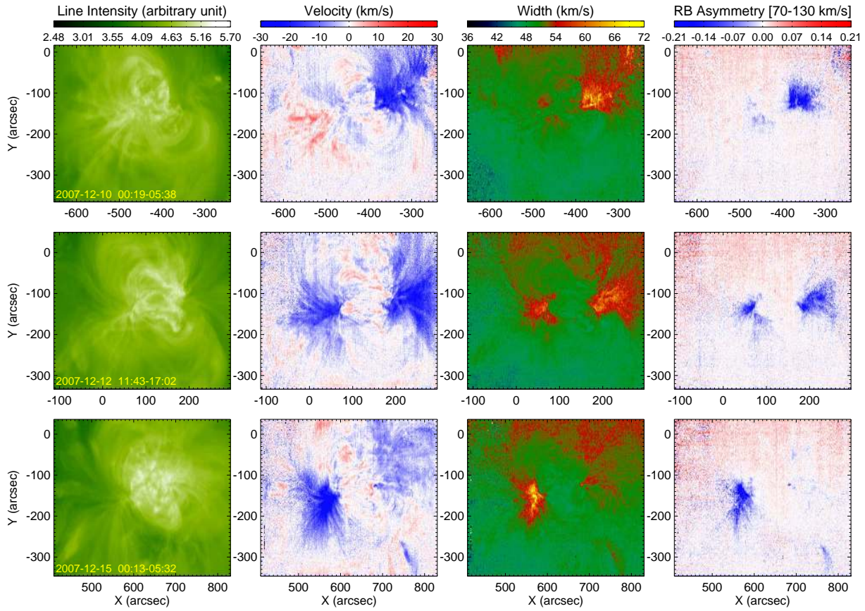
Fig. 20.— Spatial distributions of the single Gaussian parameters and profile asymmetries (averaged over the velocity interval of 70\text{--}130\text{ km s}^{-1} , as obtained from the RB_P profiles) for Fe XIII 202.04\text{\AA} in a scan from 00:19 to 05:38 on 2007 Dec 10 (first row), 11:43 to 17:02 on 2007 Dec 12 (second row), and 00:13 to 05:32 on 2007 Dec 15 (third row).
