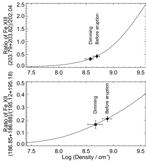
Fig. 17.— Relationship between electron density and line ratio, as derived from the CHIANTI database. The measured values before the eruption (15:11 on 2006 Dec 14) and during dimming (10:29 on 2006 Dec 15) are indicated by the solid diamonds and squares respectively. The vertical and horizontal bars indicate the standard deviations of the intensity ratios and uncertainties of the calculated densities, respectively.
