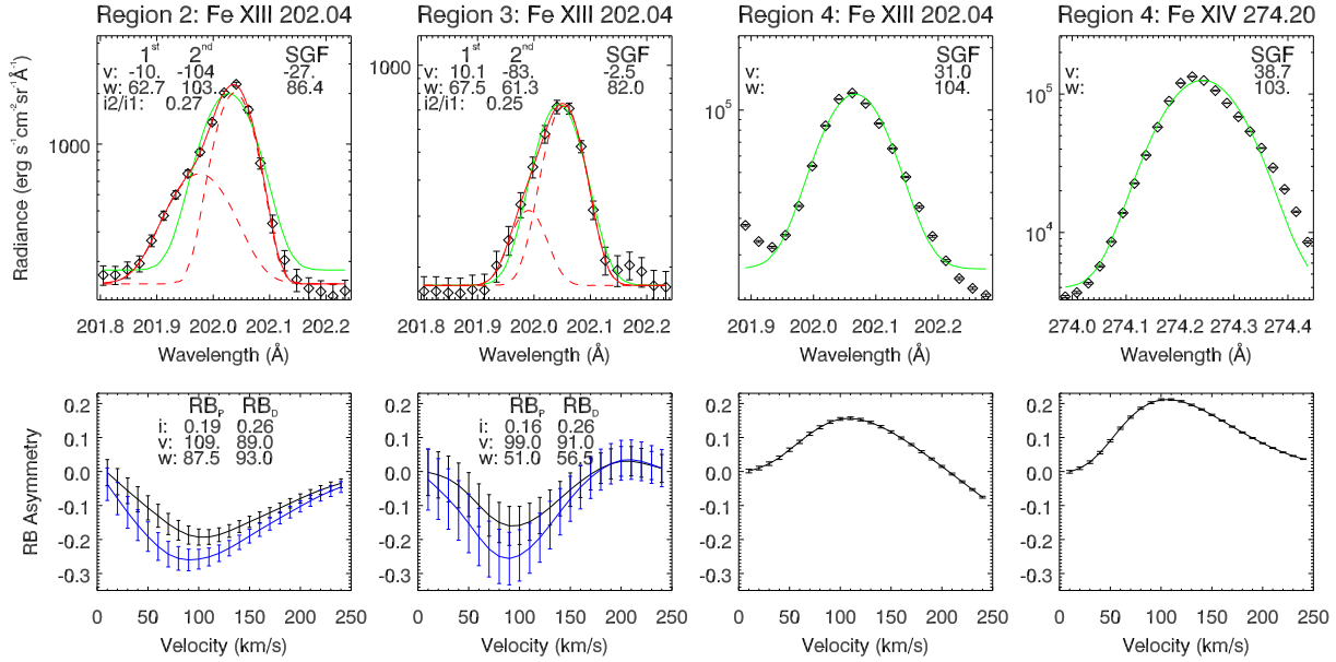
Fig. 14.— Similar to Figure 7 but for regions 2-4 marked in Figure 3. For the averaged profiles in region 4 only the single Gaussian fits and the RB P asymmetry profiles are plotted.
