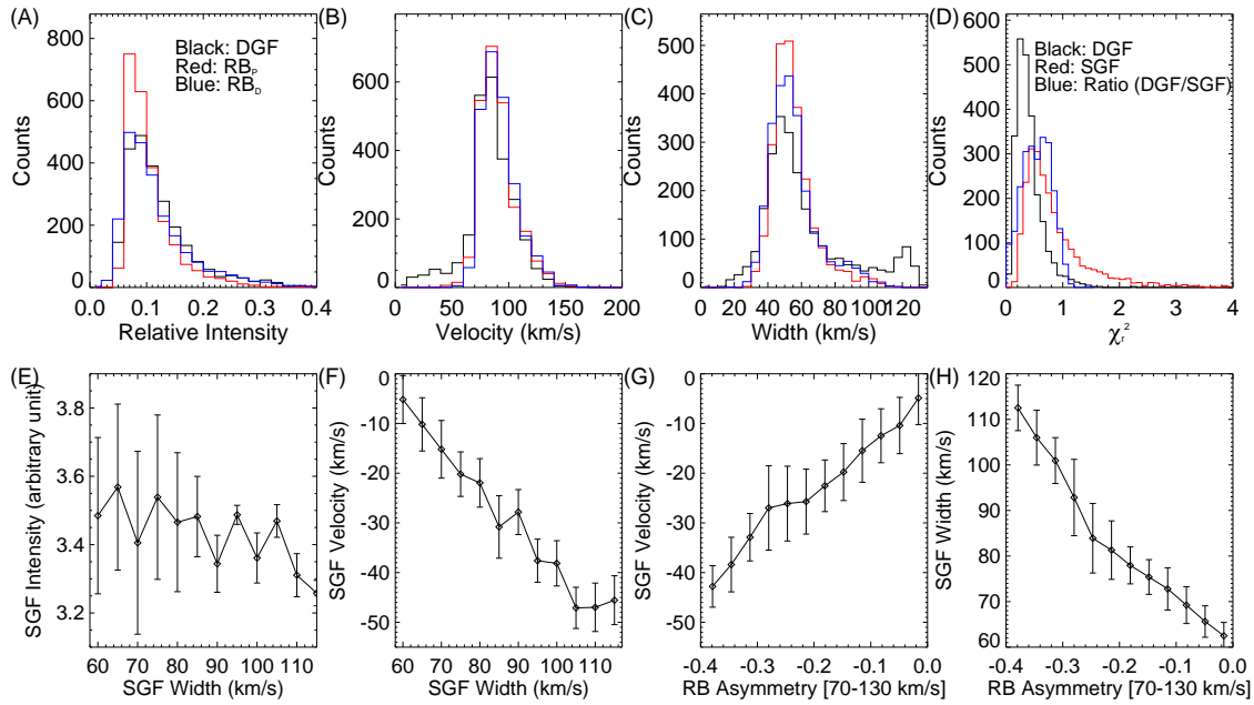
Fig. 9.— Histograms of the relative intensity (A), velocity (B), and exponential width (C) of the secondary component, as derived from double Gaussian fit (black) and RB asymmetry analysis (red/blue for RB P /RB D ) for Fe XIII 202.04 Å in the 2006 Dec 15 01:15-03:30 observation. Panel (D) shows the histograms of the \chi_r^2 values of the single (red) and double (black) Gaussian fits, as well as the ratio of the two (blue). Panels (E)&(F) show the relationship between the intensity/Doppler shift and the exponential width as derived from single Gaussian fit. Panels (G)&(H) present the relationship between the Doppler shift/exponential width derived from single Gaussian fit and the average RB P asymmetry in the velocity interval of 70-130 km s -1 .
