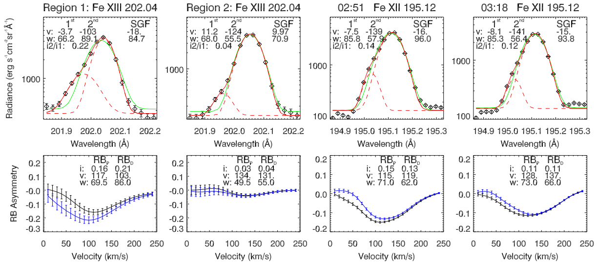
Fig. 8.— First & second columns: RB asymmetry profiles (bottom) of Fe XIII 202.04Å line profiles (top) averaged over regions 1 & 2 marked in Figure 2. Third & fourth columns: RB asymmetry profiles (bottom) of the averaged Fe XII 195.12Å line profiles (top) in dimming regions at 02:51 and 03:18 as shown in Figure 4. The line styles and denotations of parameters are the same as in Figure 7.
