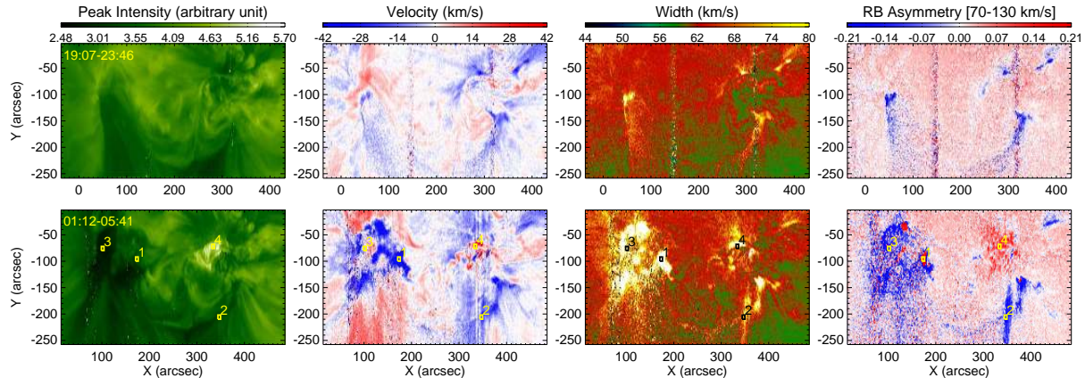
Fig. 3.— Same as Figure 1 but for the 2006 Dec 12-13 observations. The rectangular regions 1-4 mark the locations where line profiles are averaged and presented in Figures 10&14.
