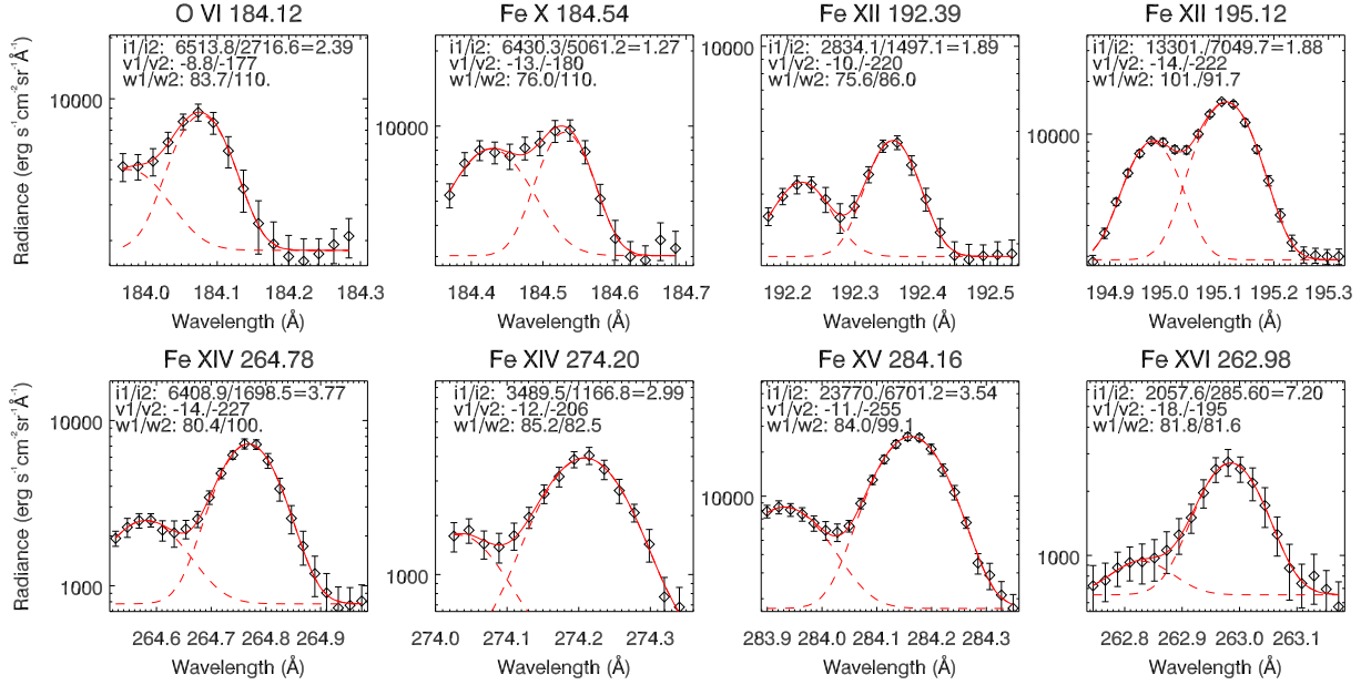
Fig. 12.— Line profiles averaged in locations marked in Figure 5. The diamonds, error bars, line styles and colors are the same as in Figure 7. The peak intensities ( i1 & i2 ), velocities ( v1 & v2 ) and exponential widths ( w1 & w2 ) of the two Gaussian components are shown in each panel.
