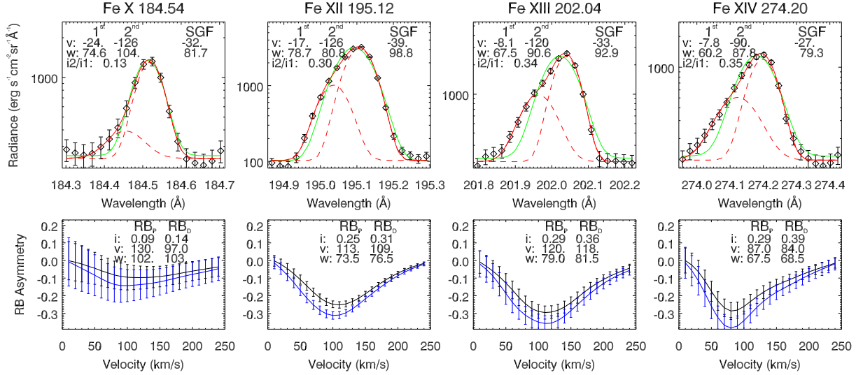
Fig. 7.— RB asymmetry profiles (bottom) of the Fe x 184.54Å, Fe XII 195.12Å, Fe XIII 202.04Å and Fe XIV 274.20Å line profiles (top) averaged over the square marked in Figure 1. Top: The observed spectra and measurement errors are shown as the diamonds and error bars, respectively. The green lines are single Gaussian fits. The two dashed red lines in each panel represent the two Gaussian components and the solid red line is the sum of the two components. The velocity (v) and exponential width (w) derived from the single (SGF) and double (1 st /2 nd for the two components) Gaussian fits are shown in each panel. Also shown is the intensity ratio of the secondary component to the primary one (i2/i1). Bottom: the black and blue lines represent RB profiles for RB P and RB D , respectively. Error bars indicate the errors propagated from the measurement errors. The peak relative intensity (i), velocity (v), and 1/e width (w) are shown in each panel.
