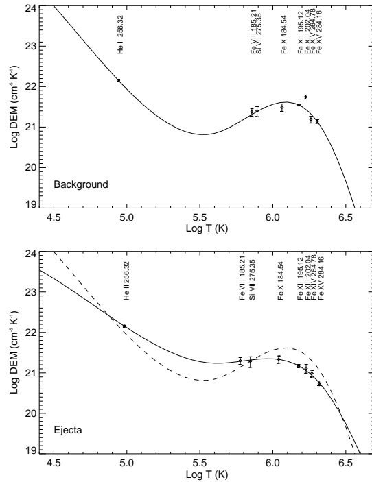
Fig. 18.— DEM curves of the background (upper panel, stationary component) and ejecta (lower panel, highly blue-shifted component) for the rectangular region marked in Figure 6. The DEM curve of the background is overplotted as the dashed line in the lower panel.
