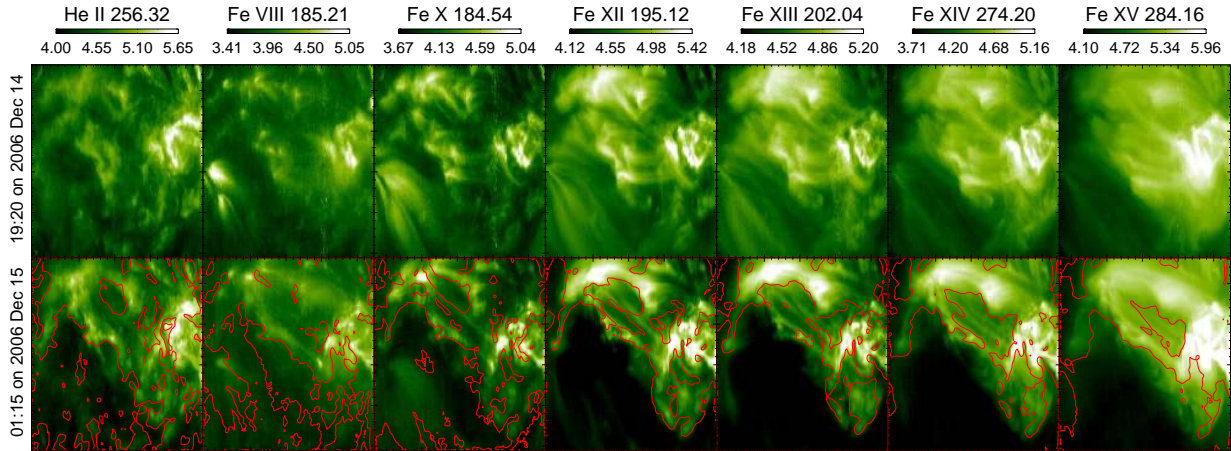
Fig. 15.— Intensity maps of different emission lines for the two scans starting at 19:20 on 2006 Dec 14 and 01:15 on 2006 Dec 15. The red contours outline regions where the intensity was significantly reduced ( \geq 20\% ).
