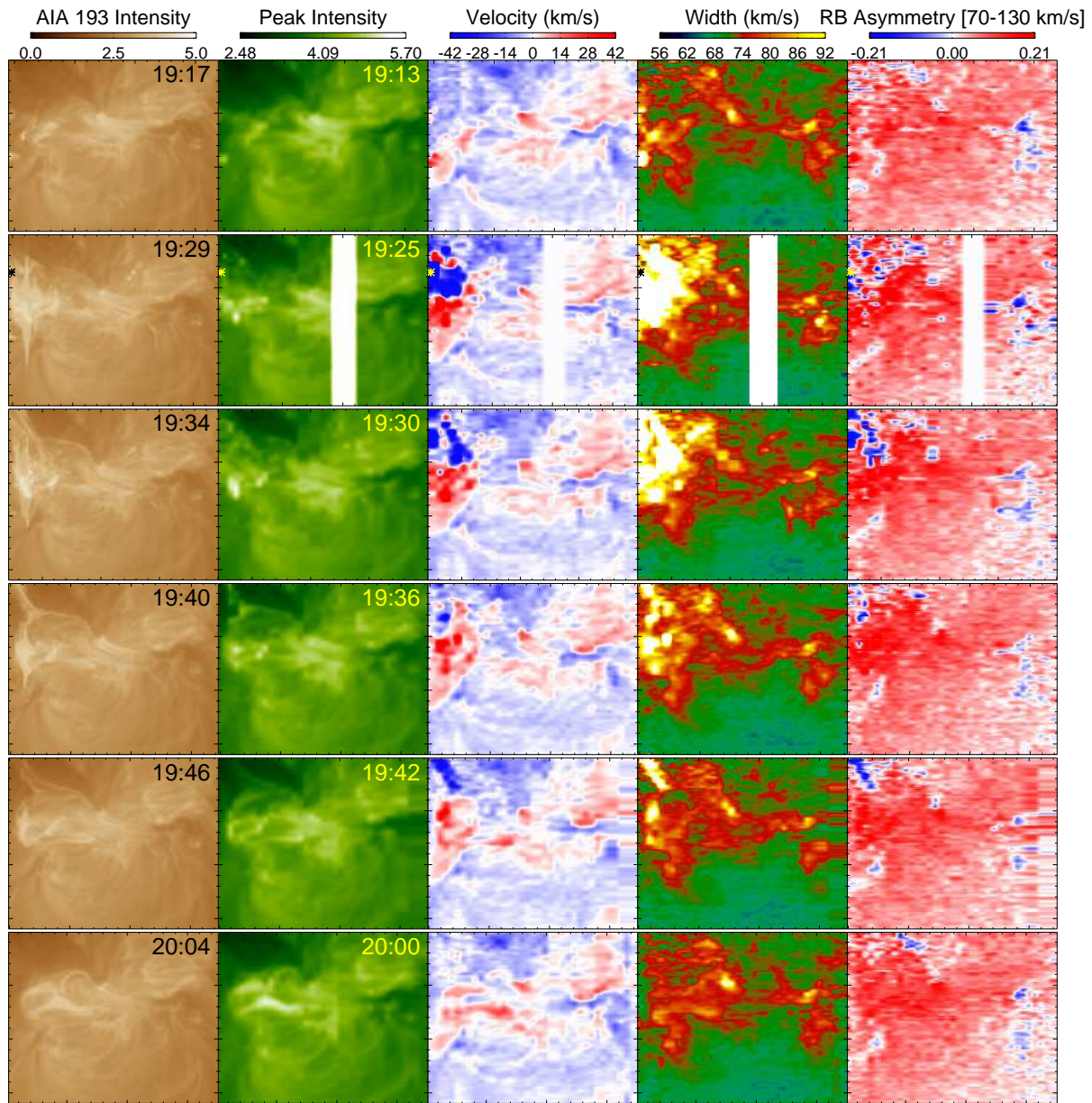
Fig. 5.— Same as Figure 4 but for the 2011 Feb 14 observations. The asterisk marks the center of five pixels along the slit where line profiles are averaged and presented in Figure 12. The size of the FOV is about 175'' \times 160'' . For illustration some bad data from single exposures are replaced by the data of adjacent exposures. A movie (m5.mpeg) showing the evolution of AIA 193Å is available online.
