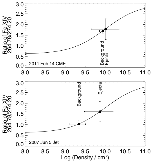
Fig. 19.— Relationship between electron density and line ratio, as derived from the CHIANTI database. The measured values for the emission of the background and ejecta are indicated by the solid diamonds and squares respectively. The error bars indicate uncertainties of the ratios and densities as calculated from the 1\text{-}\sigma uncertainties of the double Gaussian fit intensities. Upper: the 2011 Feb 14 CME; Lower: the 2007 Jun 5 jet.
