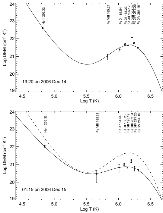
Fig. 16.— DEM curves for the two scans starting at 19:20 on 2006 Dec 14 (upper panel, before eruption) and 01:15 on 2006 Dec 15 (lower panel, dimming). The DEM curve before the eruption is overplotted as the dashed line in the lower panel.
