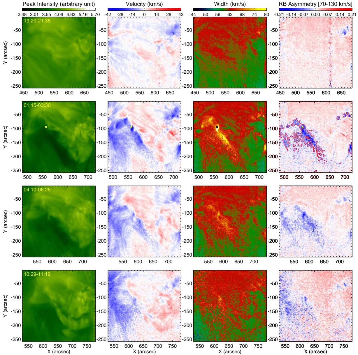
Fig. 1.— Spatial distributions of the peak intensity, Doppler velocity and exponential width derived from the single Gaussian fit, and the average RB_P asymmetry in the velocity interval of 70\text{--}130\text{ km s}^{-1} for Fe XIII 202.04\text{\AA} in the 2006 Dec 14-15 observations. The beginning and ending time (hour:minute) of each scan is indicated in the intensity image. The pre-eruption conditions are shown in the first row. The square in each panel of the second row marks locations where profiles are averaged and presented in Figure 7. The red contours shown in the map of RB_P asymmetry for the 01:15-03:30 scan outline locations where the RB_P asymmetry ( 70\text{--}130\text{ km s}^{-1} ) is smaller than -0.03 and the signal to noise ratio of the profile is larger than 8.
