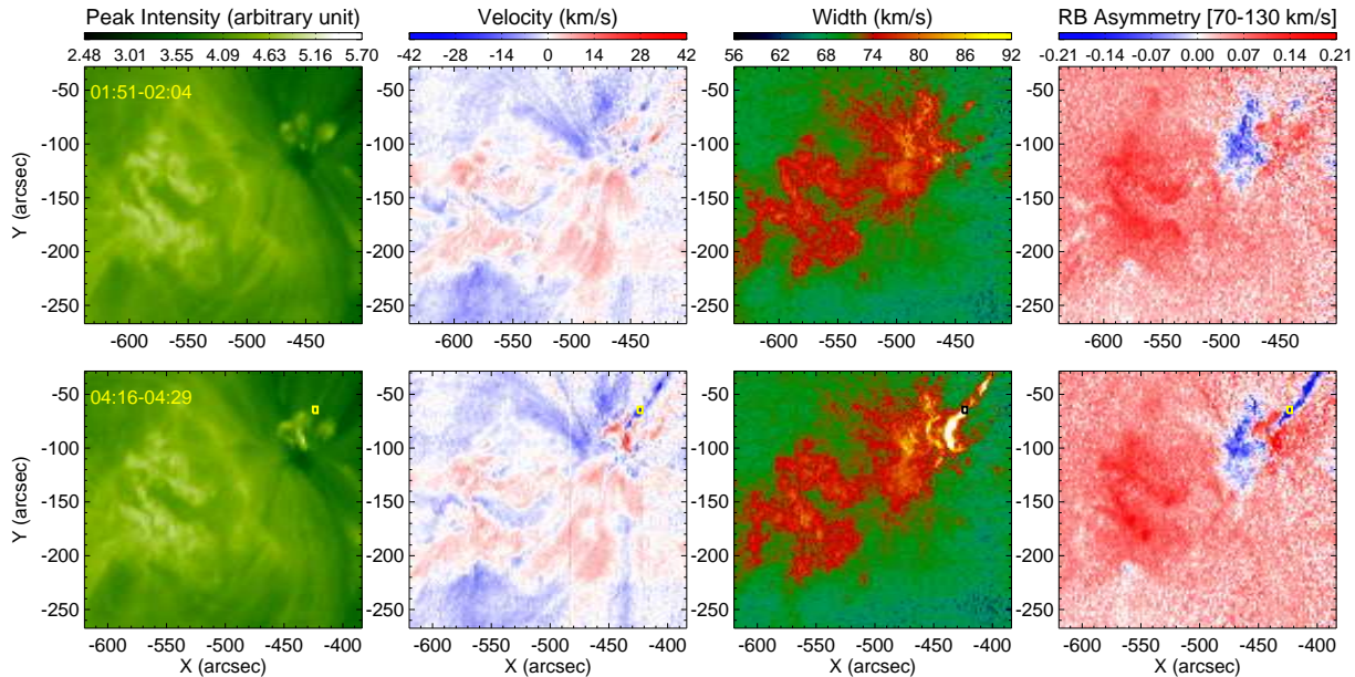
Fig. 6.— Same as Figure 1 but for Fe XII 195.12Å in the 2007 Jun 5 observations. The rectangular region marks the locations where line profiles are averaged and presented in Figure 13.
