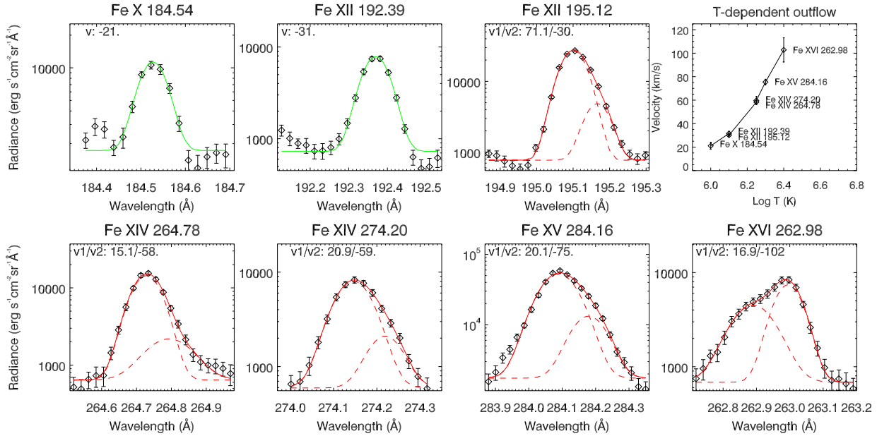
Fig. 11.— Same as Figure 10 but for the rectangular region marked in Figure 4.
