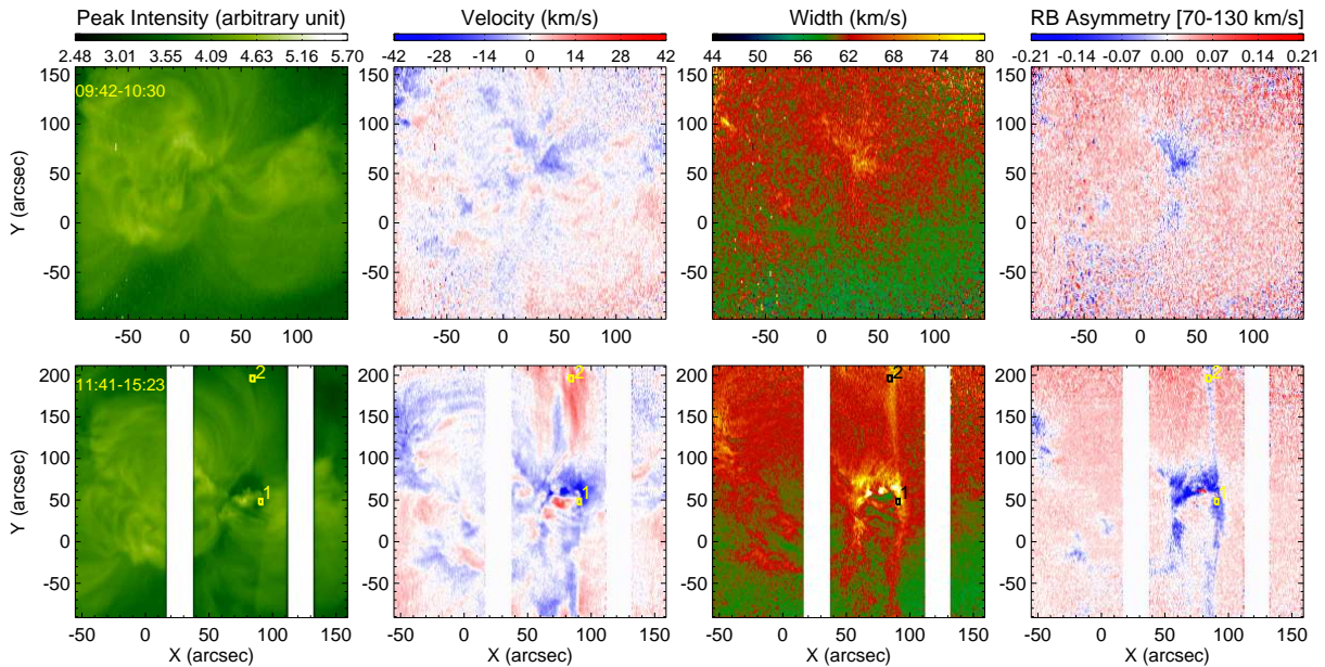
Fig. 2.— Same as Figure 1 but for the 2007 May 19 observations. The rectangular regions 1 & 2 mark the locations where the Fe XIII 202.04Å profiles are averaged and presented in Figure 8.
