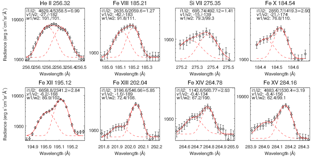
Fig. 13.— Same as Figure 12 but for the rectangular region marked in Figure 6.
