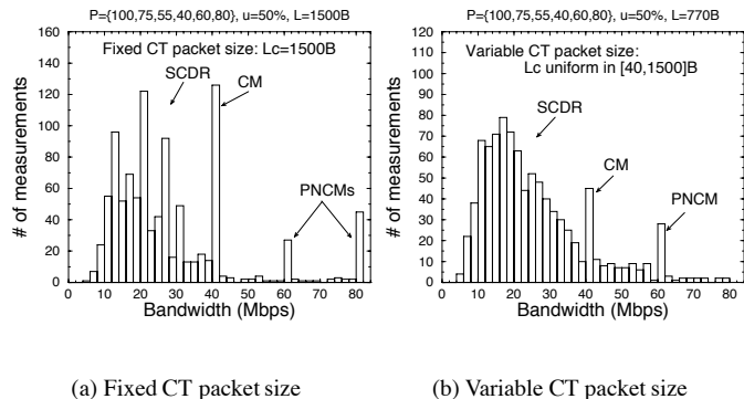
Fig. 5. Fixed versus variable CT packet size L_c .
