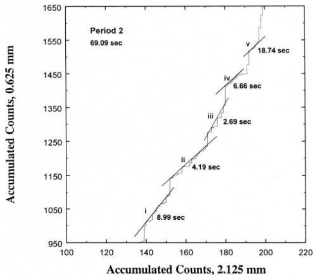
FIG. 6. Accumulated counts of 0.625-mm-diameter drops are plotted as a function of accumulated counts of those at 2.125-mm diameter for video disdrometer observations in rain. There are several regions or patches of linear relations between the two counts consistent with the presence of steady drop size distributions. Also note the slopes of the lines change indicating that the “slopes” of the distributions themselves are different for each patch (from Jameson and Kostinski 2000).
