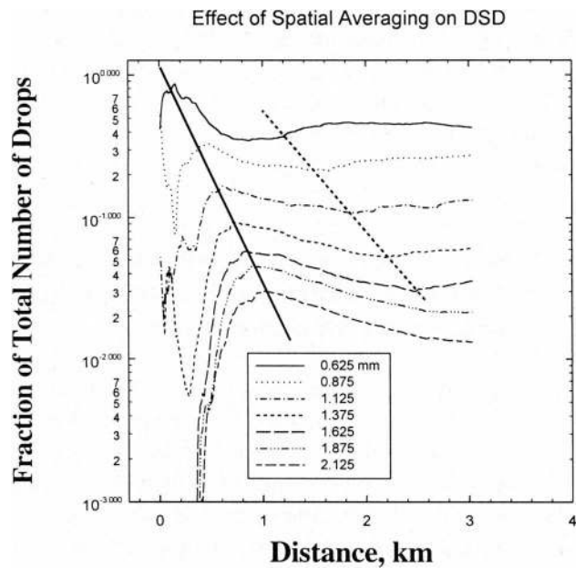
FIG. 2. Fractions of the total number of drops as functions of increasing sample pathlength (sample size) for the seven indicated drop size categories corresponding to Fig. 1 as discussed in the text. Note that the distributions never become steady (i.e., simultaneously horizontal at all sizes.)
