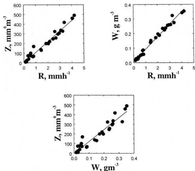
FIG. 8. Scatterplots between different average powers of the diameter (zero moments) observed during the first 29 samples in Fig. 1. Linearity between such moments may be useful as an indicator of statistical homogeneity.
