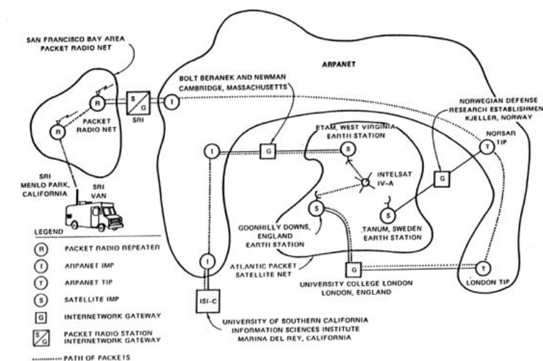
Figure 1. A diagram of ARPANET from the 1980s
