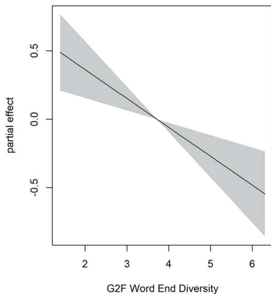
Figure 9. Partial effect of G2F Word End Diversity on the probability of choosing the -a genitive form.
