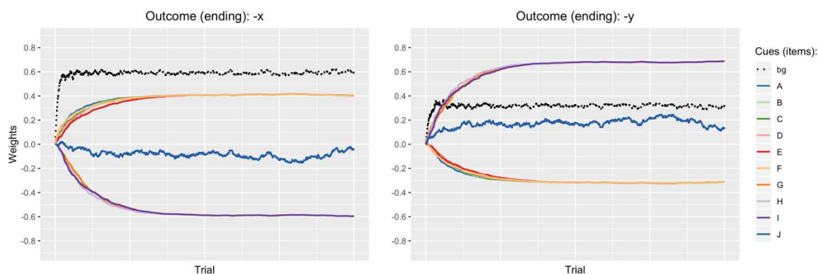
Figure 3. Simulation of learning a phenomenon that combines rules and probabilities.
