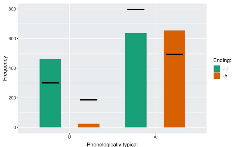
Figure 4. Plot of observed versus predicted frequencies for PhonologicallyTypical.
