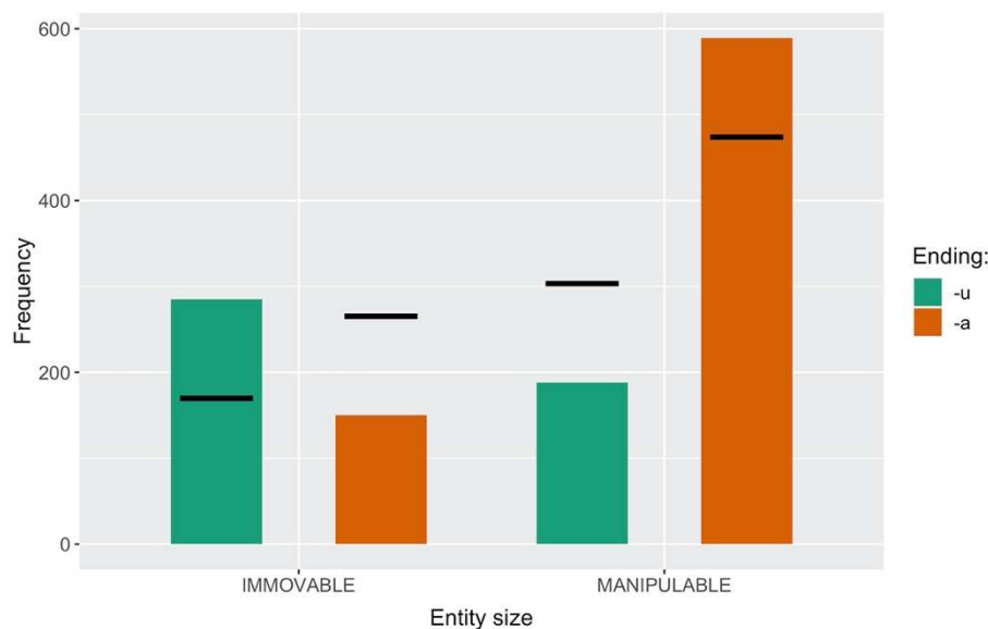
Figure 7. Plot of observed versus predicted frequencies for EntitySize.
