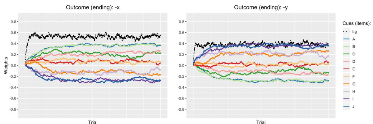
Figure 2. Simulation of learning a probabilistic phenomenon.
