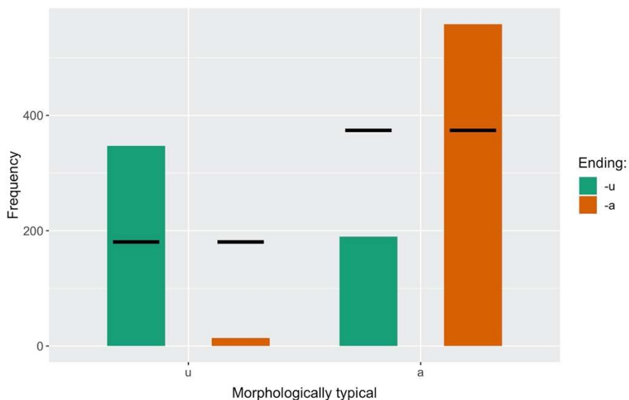
Figure 5. Plot of observed versus predicted frequencies for MorphologicallyTypical.
