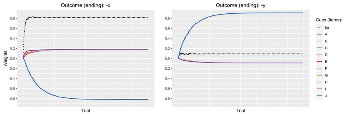
Figure 1. Simulation of learning a rule-based phenomenon with an exception.
