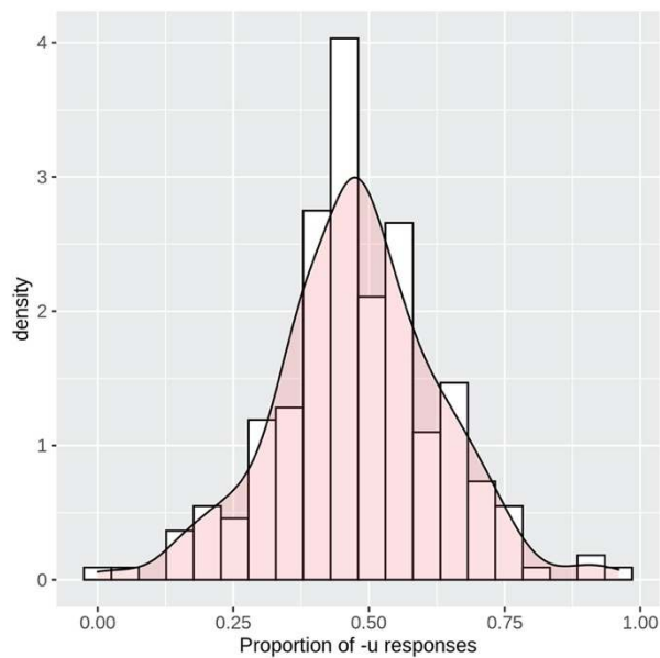
Figure 10. Histogram of the distribution of the -u response proportions from participants and its probability density function estimate.
