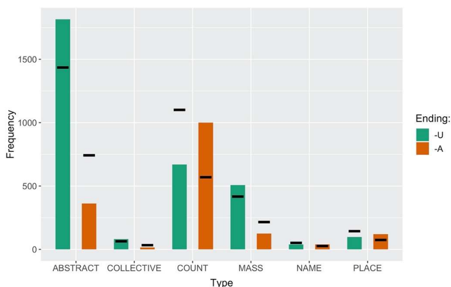
Figure 6. Plot of observed versus predicted frequencies for Type.
