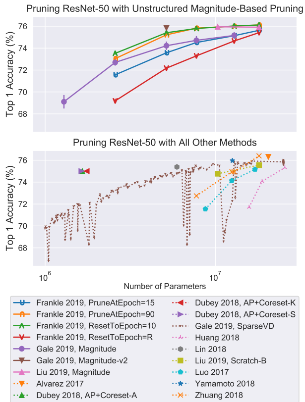
Figure 5: Pruning ResNet-50 on ImageNet. Methods in the upper plot all prune weights with the smallest magnitudes, but differ in implementation, pruning schedule, and fine-tuning. The variation caused by these variables is similar to the variation across different pruning methods, whose results are shown in the lower plot. All results are taken from the original papers.
