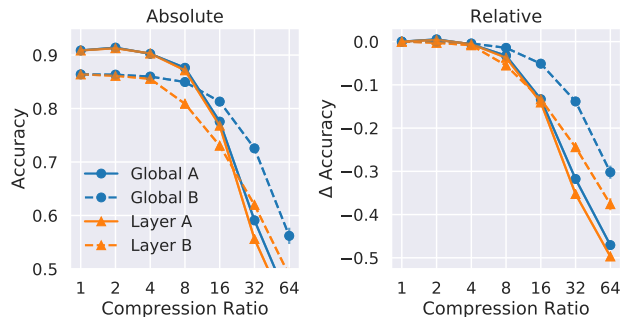
Figure 8: Global and Layerwise Magnitude Pruning on two different ResNet-56 models. Even with all other variables held constant, different initial models yield different tradeoff curves. This may cause one method to erroneously appear better than another. Controlling for initial accuracy does not fix this.
