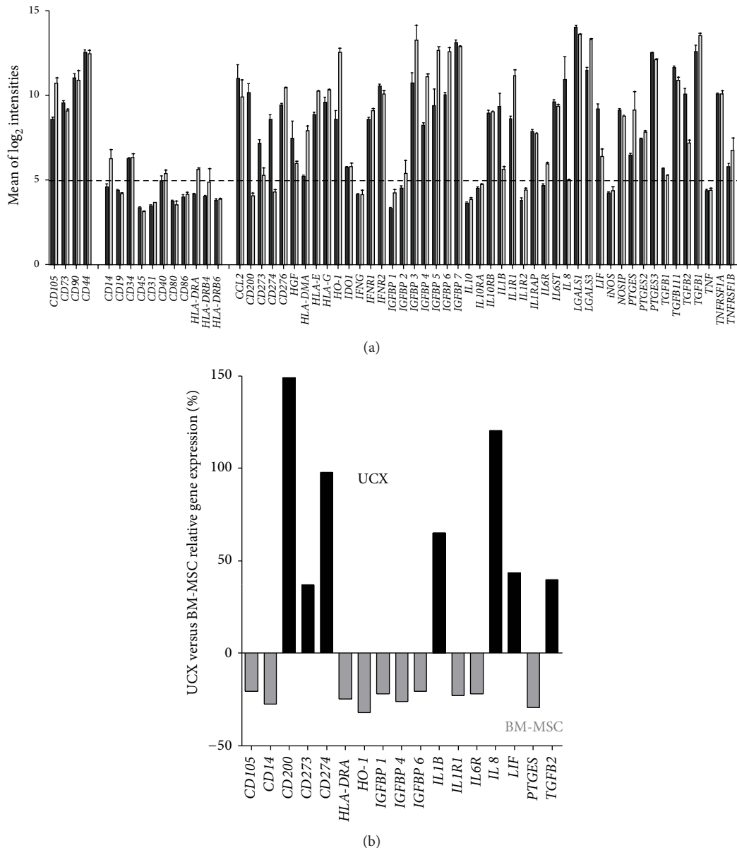
FIGURE 5: Comparison of UCX (black bars) and BM-MSCs (grey bars) transcriptome of immunomodulatory genes. (a) Relative gene expression of known MSC and immune response related genes in UCX (derived from 3 different umbilical cords) and BM-MSCs (2 different donors) are represented as mean \pm s.e.m. Unbroken line was positioned on the average negative known markers of MSCs. Genes with relative expression values above this line were considered substantially expressed. (b) Genes where there was a relative expression significantly increased or decreased 20% or more.
