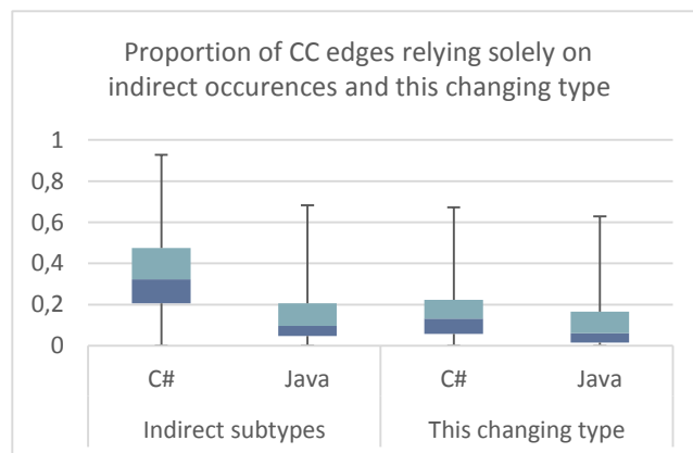
Figure 13: Proportion of CC edges relying solely on indirect subtype occurrences (left) and edges relying solely on occurrences of this changing type (right).
