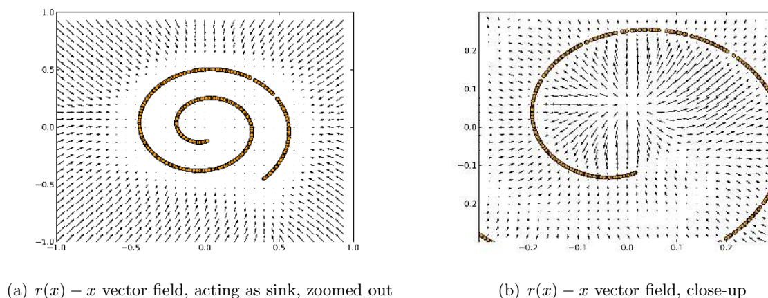
Figure 5: The original 2-D data from the data-generating density p(x) is plotted along with the vector field defined by the values of r(x) - x for trained auto-encoders (corresponding to the estimation of the score \frac{\partial \log p(x)}{\partial x} ).
