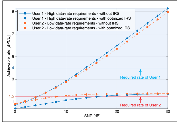
Fig. 2. Achievable rates versus SNR for MIMO-NOMA and IRS-NOMA systems under fixed power allocation where user 1 is located at 200 m and user 2 at 100 m from the BS. The power allocation coefficients of users 1 and 2 are 7/10 and 3/10 , respectively.
