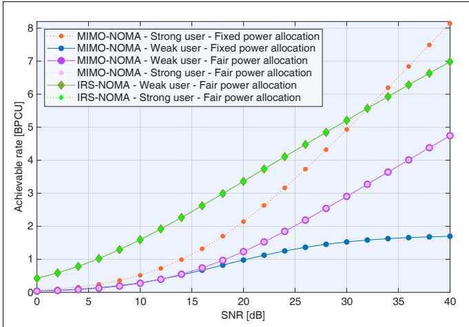
Fig. 3. Achievable rates versus SNR for MIMO-NOMA and IRS-NOMA systems under fixed and fair power allocation, where the weak user is located at 200 m and the strong one at 100 m from the BS. When fixed allocation is employed, the power coefficients for the weak and strong users are 7/10 and 3/10, respectively.
