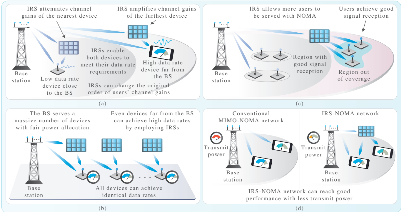
Fig. 1. Illustration of potential achievements of IRS-NOMA networks. (a) The IRSs can tune the channel gains to meet the data rate requirements of both near and far users. (b) The IRSs can boost the performance of the network under fair resource allocation. (c) By deploying an IRS at the cell-edge, more users can be served with NOMA. (d) The IRS-NOMA system can achieve similar rate performance of conventional MIMO-NOMA with less transmit power.
