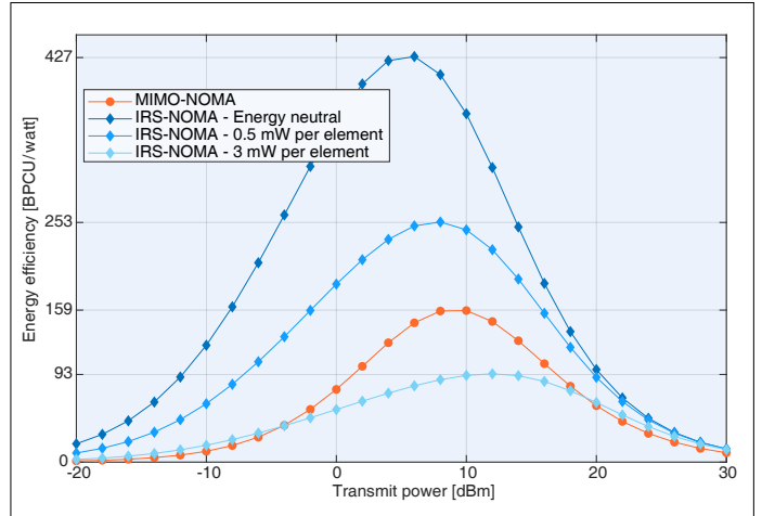
Fig. 5. Energy efficiency versus transmit power for MIMO-NOMA and IRS-NOMA systems under fixed power allocation. Two users are considered in this simulation, one located at 100 m and another at 200 m from the BS. The power coefficients for the far and near users are 7/10 and 3/10, respectively.
