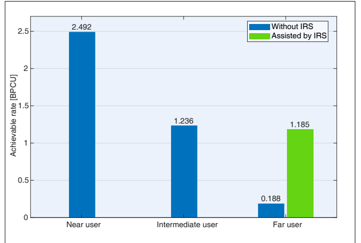
Fig. 4. Achievable rates when the SNR is 26 dBm for MIMO-NOMA and IRS-NOMA systems serving three users with fixed power allocation. The near user is located at 100 m, the intermediate user at 200 m, and the far user at 1500 m from the BS. The power coefficients for the near, intermediate, and far users are 1/10, 3/10 and 6/10, respectively.
