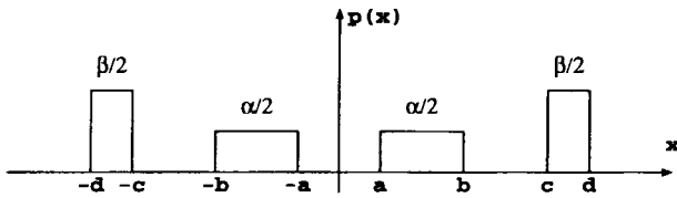
Fig. 1. Example of x -limited pdf.
