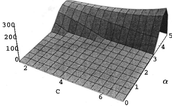
Fig. 2. Representation of K^*(p(x)) according to parameters c and \alpha , with a = 0.9 , b = 1.1 , and d = 9 .
