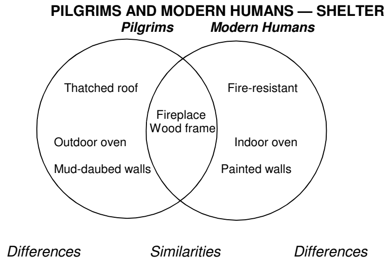
ILLUSTRATION 3.1: VENN DIAGRAM
