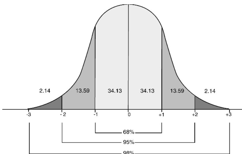
Figure 1.1: Normal Distribution
