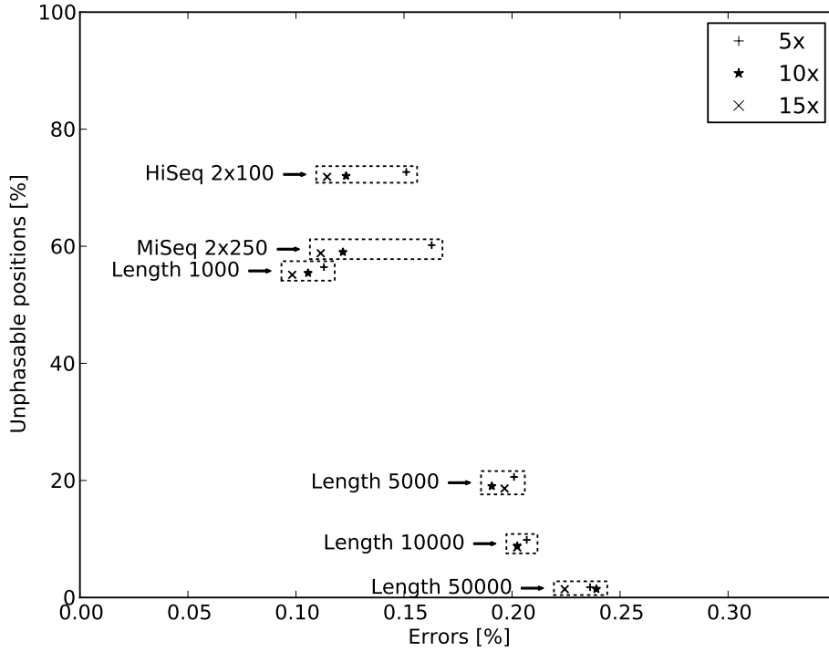
Figure 2: Performance of phasing human chromosome 1 with 68 184 heterozygous SNPs in total using different simulated data sets and different coverages. The unphasable positions percentage (y-axis) gives the fraction of the SNP positions that could not be phased due to not being covered by reads that span more than one SNP position. The x-axis shows the percentage of all SNPs that were not unphasable but wrongly phased by the algorithm, either because of a flip error, a switch error, or due to being reported as an ambiguous position by WHATSHAP. Length 1 000, 5 000, 10 000, and 50 000 refer to reads of this length from a hypothetical sequencer with an error rate of 1%. HiSeq/MiSeq refers to using error profiles specific to these instruments during read sampling. Data sets are pruned to three different target coverages (5x, 10x, 15x) encoded by different symbols in the plot (see legend).
