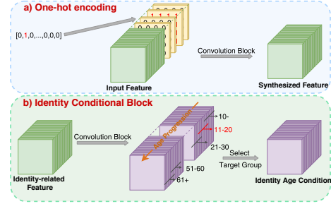
Figure 3: Comparison between one-hot encoding and ICB.
