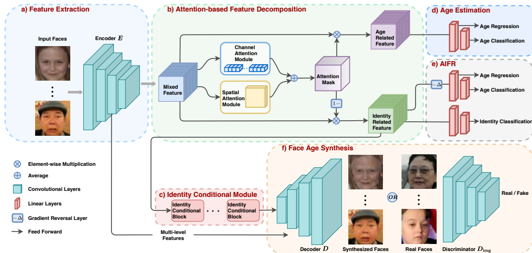
Figure 2: An overview of the proposed MTLFace including two tasks. AIFR: The encoder E first extracts the mixed feature maps from input faces, which are then decomposed into two disjoint identity- and age-related feature maps by the multi-task training and continuous domain adaption. FAS: The decoder D produces synthesized faces through identity conditional module based on multi-level features; the PatchDiscriminator D_{img} penalizes the framework for better visual quality.
