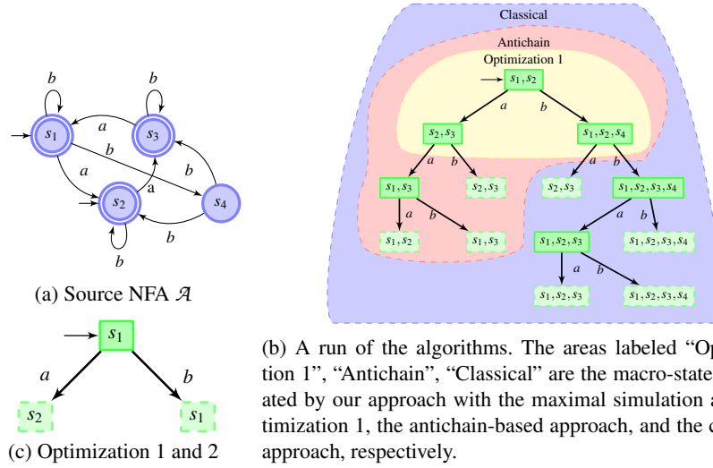
Fig. 1. Universality Checking Algorithms
