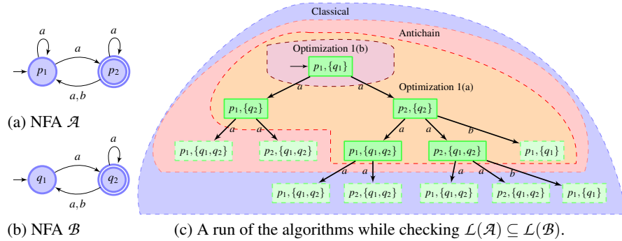
Fig. 2. Language Inclusion Checking Algorithms
