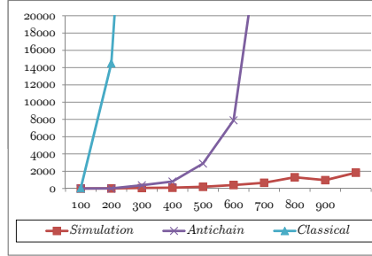
(b) Language inclusion always holds
