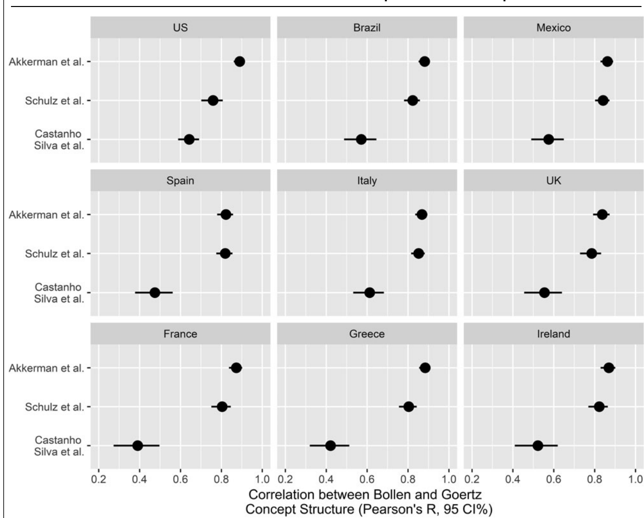
FIGURE 5. Correlations Between Goertz and Bollen Concept Structures of Populist Attitudes
