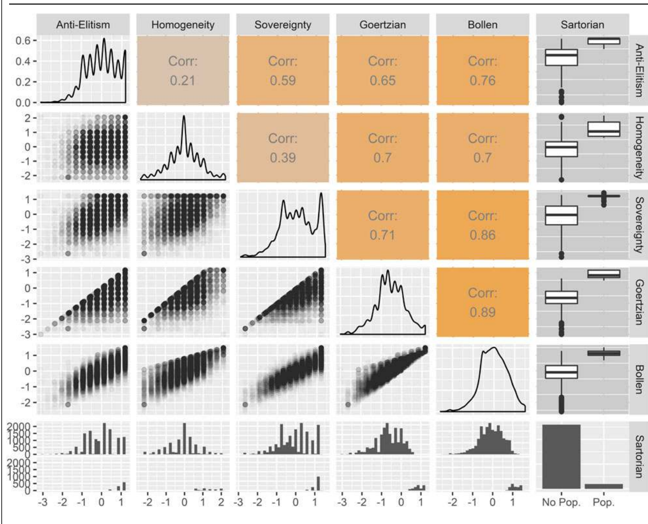
FIGURE 2. Distributions of and Correlations Between Concept Structures of Populist Attitudes and Concept Attributes (Germany, Schulz et al. Populism Scale)
