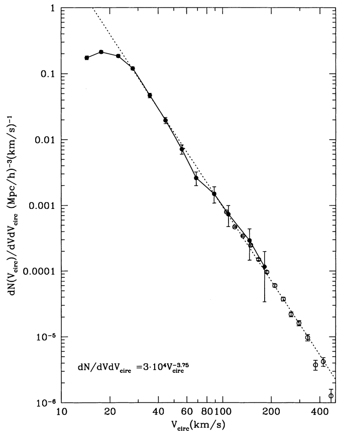
FIG. 1.—Differential circular velocity distribution function of DM halos in the \Lambda CDM model. The solid curve and the filled circles are results of the small box (box size of 7.5 h^{-1} \text{ Mpc} ) simulation. Open circles show the corresponding velocity function in a larger (box size of 60 h^{-1} \text{ Mpc} ) simulation. Error bars correspond to the Poisson noise. The dotted curve is the power law with the slope of -3.75 motivated by the Press-Schechter approximation (see § 4 for details).
