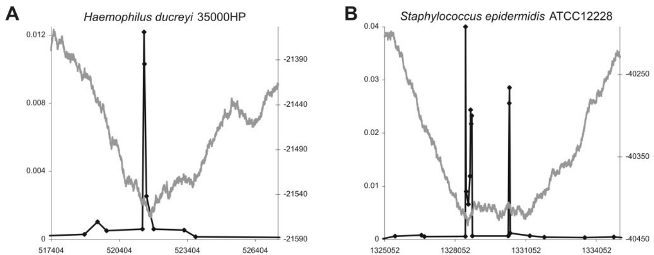
Figure 3. DNA asymmetry in [G–C], DnaA boxes' distribution and dnaA gene location in the oriC region. Example of single cluster of DnaA boxes (A) and a few separated clusters in the region (B). See Figure 1 for further explanation.
