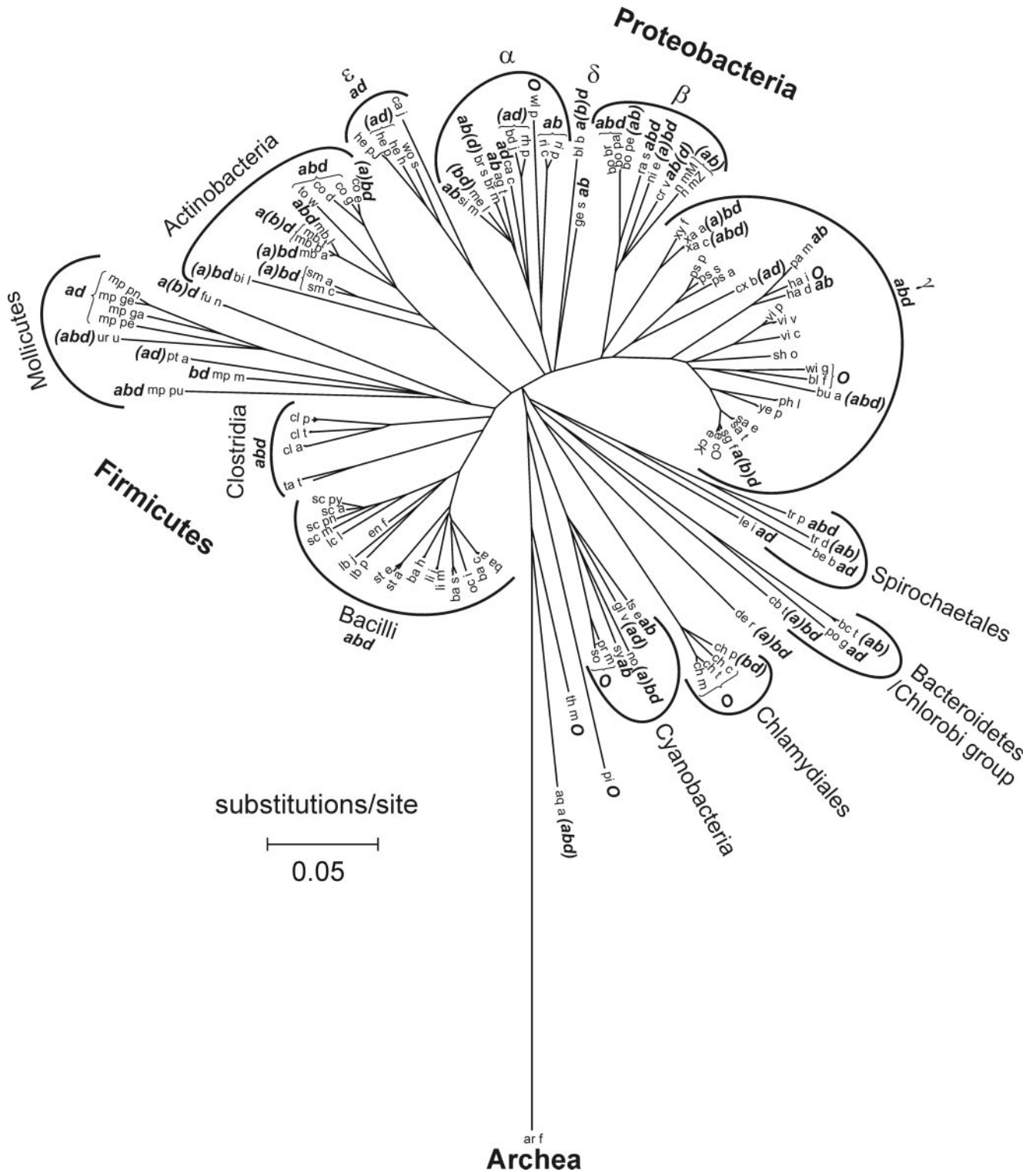
Figure 5. The 16S rRNA phylogenetic tree for 112 analysed bacteria and their classification based on concordance of methods of oriC identification: DNA asymmetry, DnaA box distribution and the dnaA gene location. The tree was built with the minimum evolution method (ME) by the MEGA 2.1 program (42) assuming the Tamura–Nei model of nucleotide substitutions (43). Abbreviations of the bacterial names are listed in Supplementary Table 1. Archaeoglobus fulgidus (ar f) was chosen as representative of the Archaea.
