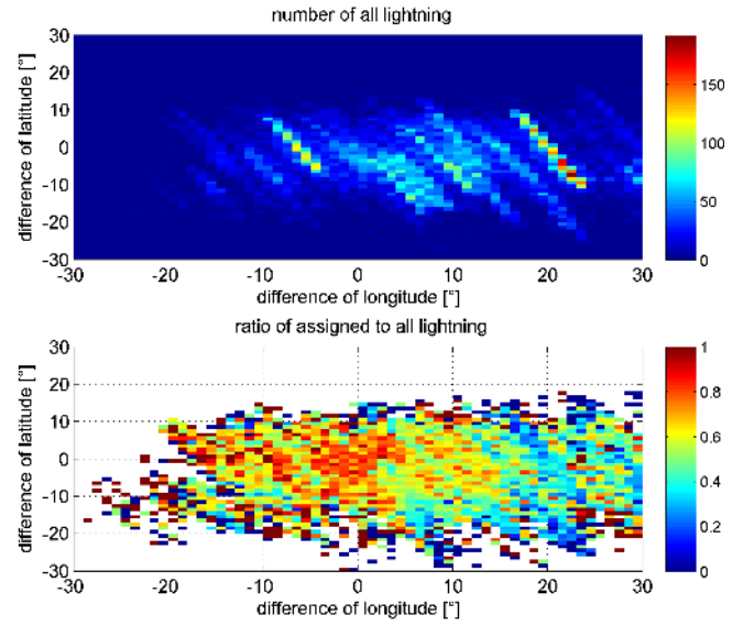
Fig. 5. Top: number of all lightning detected by the EUCLID network as a function of longitudinal and latitudinal difference between the magnetic footprint and locations of lightning. Bottom: Ratio of the assigned to all lightning (nighttime cases).
