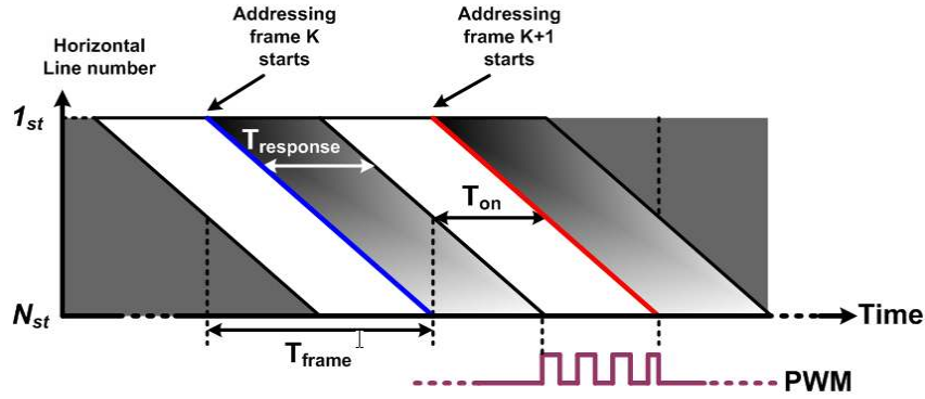
Fig. 6 T_{on} determination on the backlight scanning idea.
