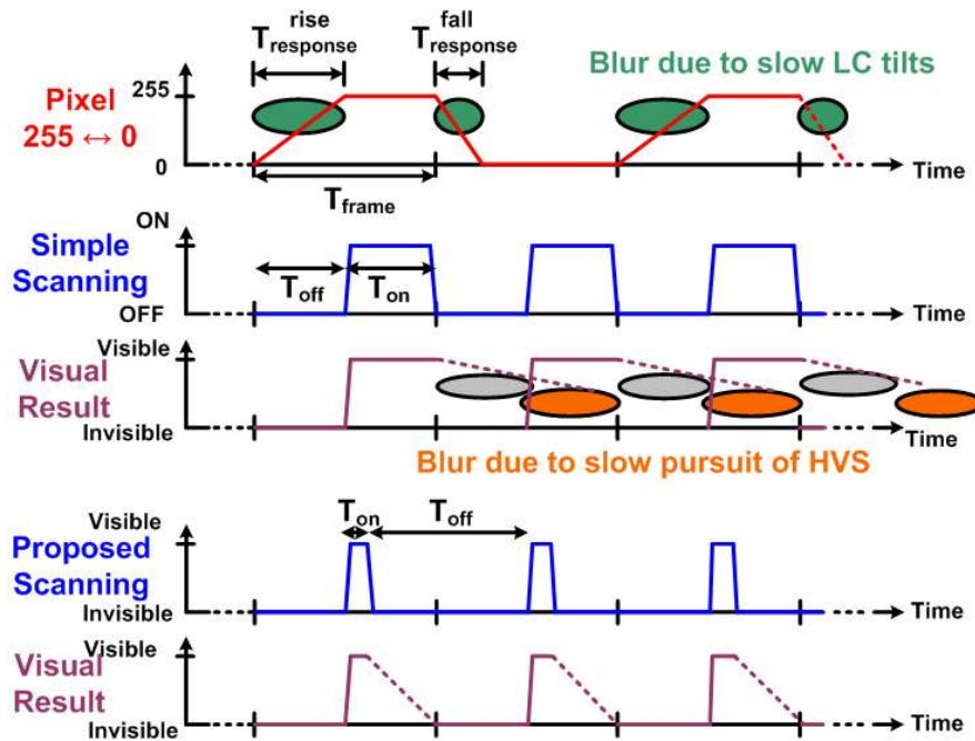
Fig. 7 Proposed 1-D LED backlight scanning idea.
