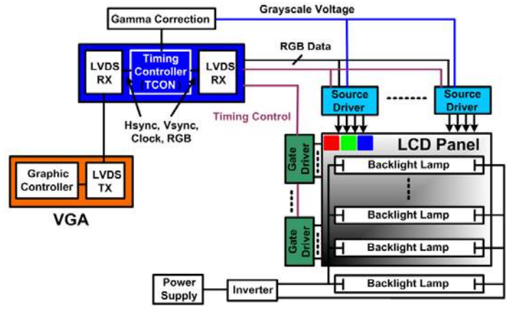
Fig. 3 Circuit architecture for LCD panel driving.
