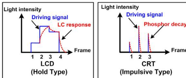
Fig. 1 Hold-type image display in LCD vs. impulse-type image display in CRT.
