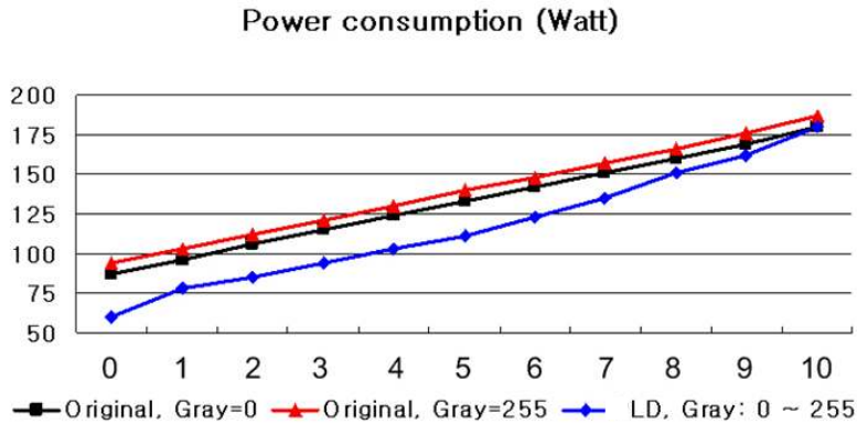
Fig. 12 Power consumptions in the ‘Original’ vs. ‘LD’.
