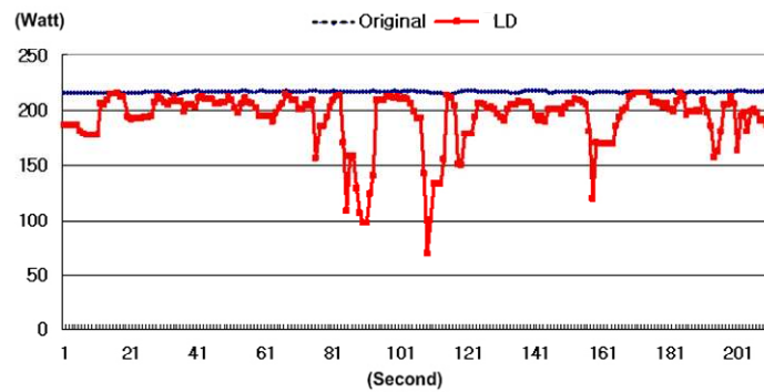
Fig. 13 Power consumption of the ‘Iron Man’.
