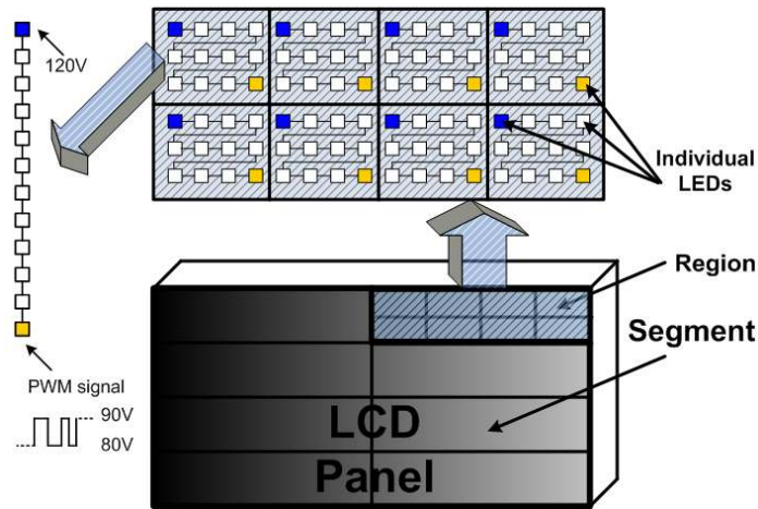
Fig. 9 LED arrangement in LCD Panel.
