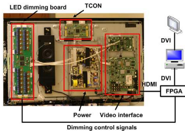
Fig. 2 Test Environment and circuit blocks on the panel.
