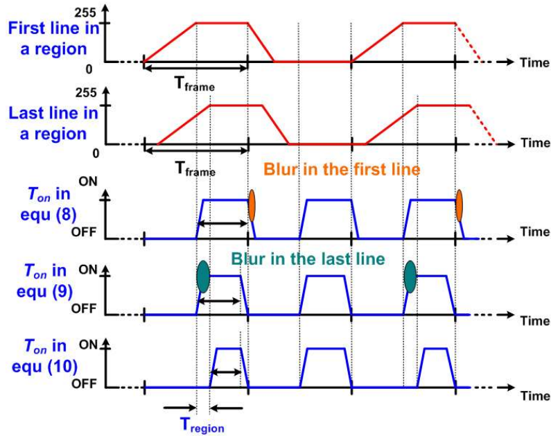
Fig. 8 Determination of the turn-on time of LEDs.
