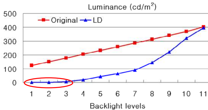
Fig. 11 Luminance changes in the ‘Original’ vs. ‘LD’.
