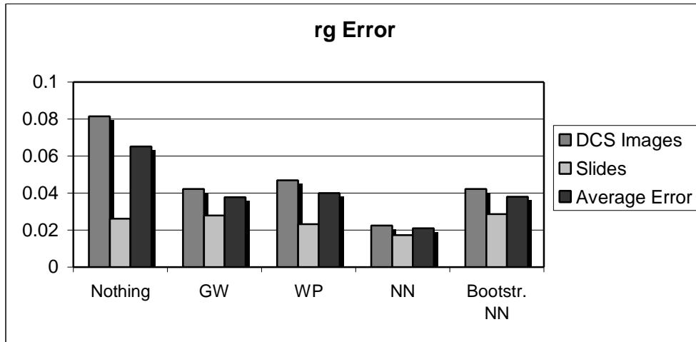
Figure 2. Average errors measured in rg-chromaticity space.
