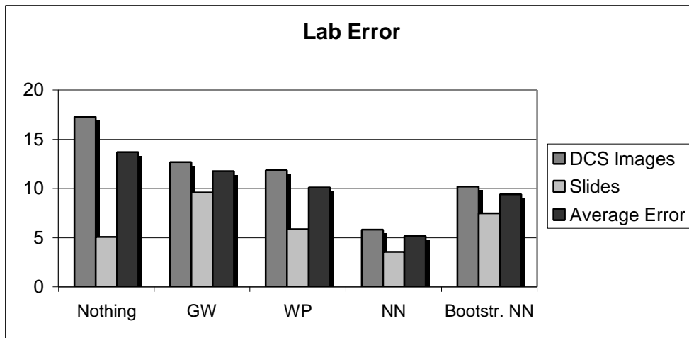
Figure 3. Average CIE Lab \Delta E space between actual and estimated illuminant fixed to the same L^* value.
