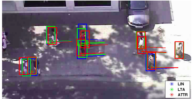
Figure 3. Tracker example. The line indicates the displacement from the previous frame. Under 0.625 fps, it is hard to find a correspondence between frames without prior.
